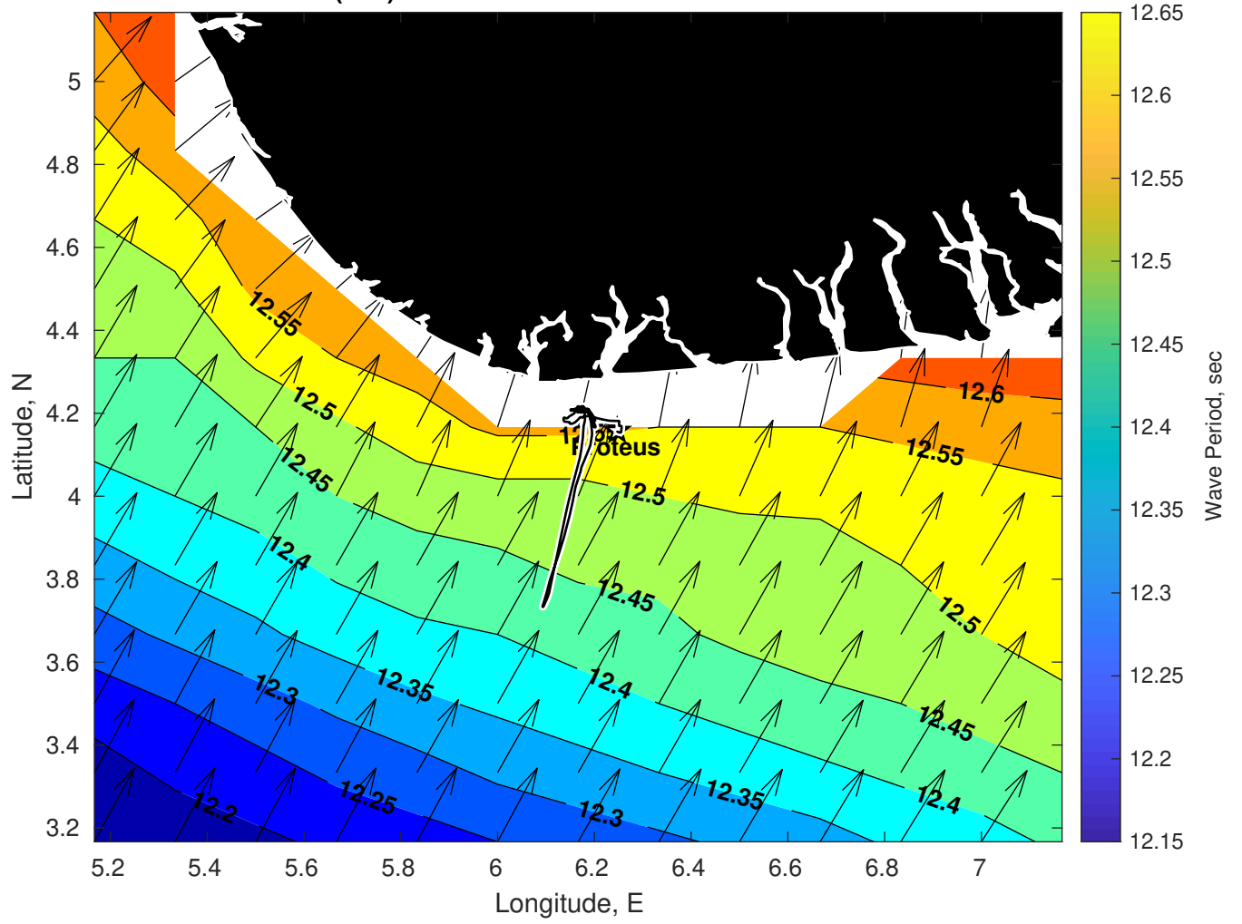
Wave Period (sec) for Proteus at 29-Jan-2025 09:00:00
