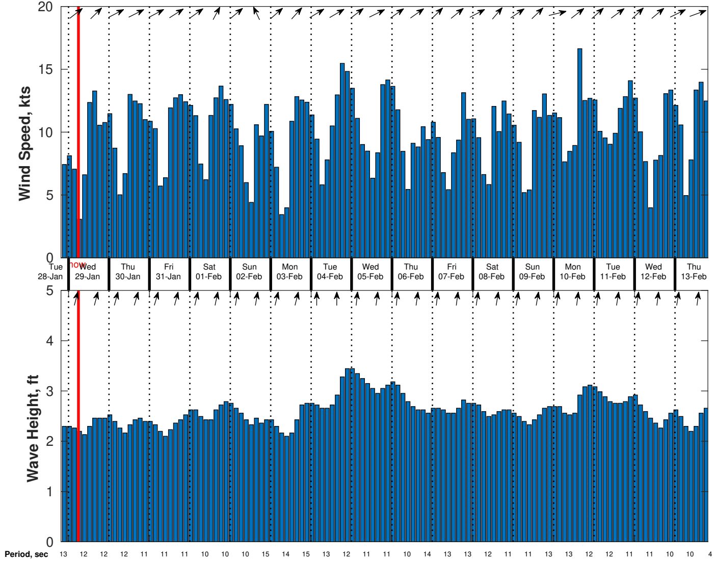
Wind & Wave Forecast for Proteus from 28-Jan-2025 20:00:00 to 13-Feb-2025 20:00:00
