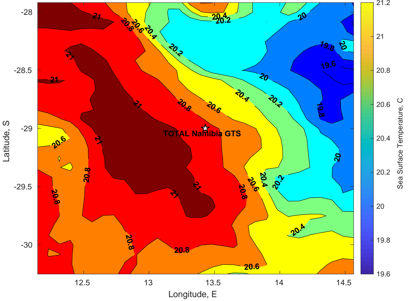
SST for TOTAL Namibia GTS at 28-Jan-2025 00:00:00
