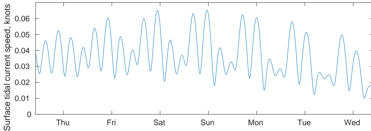
Tidal Currents and Heights for TOTAL Namibia GTS at 20250129
