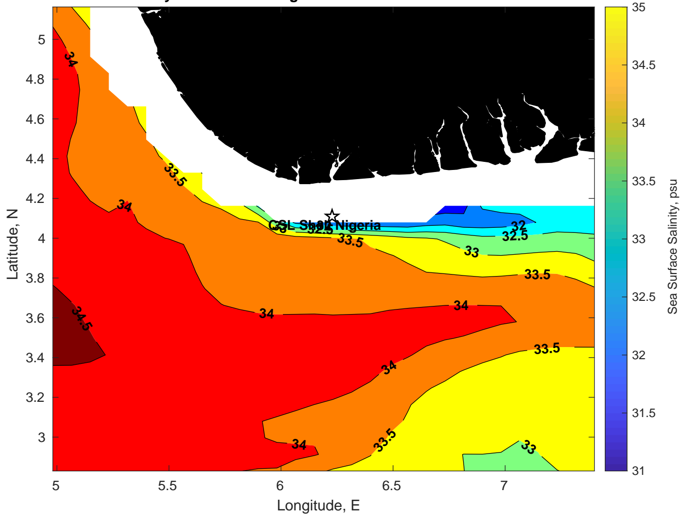
Surface Salinity for CSL Shell Nigeria at 29-Jan-2025 00:00:00
