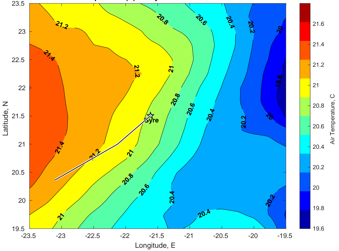
Air Temperature (C) for Gyre at 30-Jan-2025
