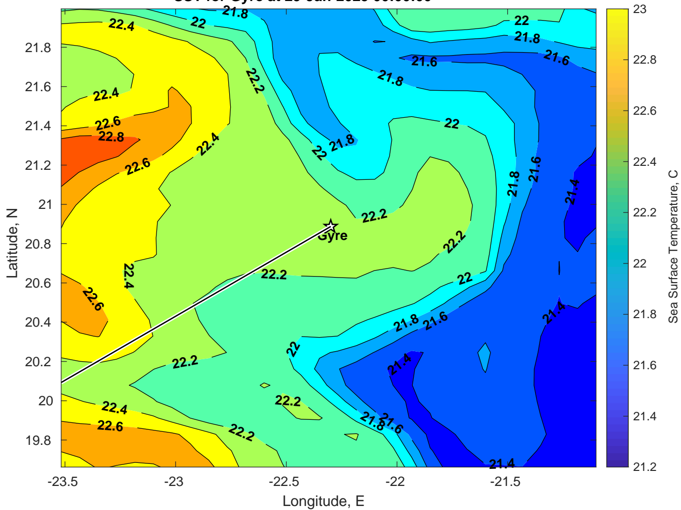
SST for Gyre at 29-Jan-2025 00:00:00
