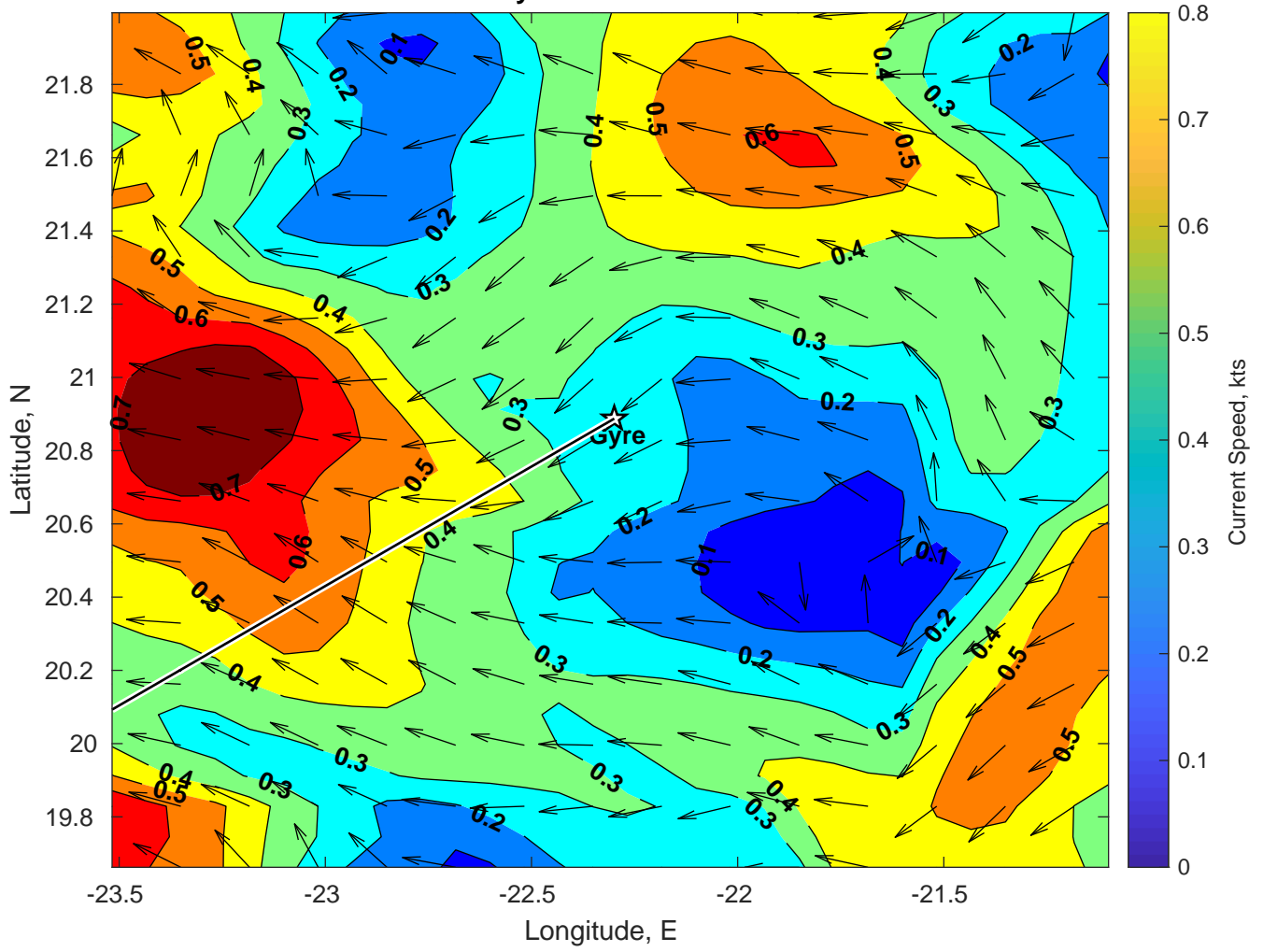
Surface Currents for Gyre at 29-Jan-2025 00:00:00
