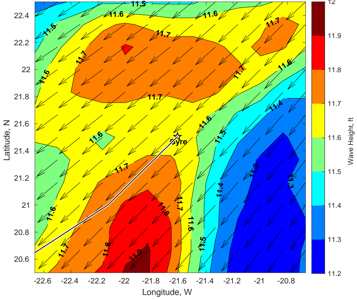
Wave Height (ft) for Gyre at 30-Jan-2025 09:00:00
