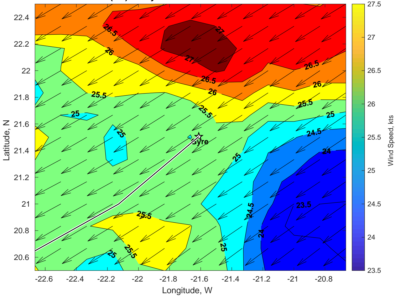
Winds (kts) for Gyre at 30-Jan-2025 09:00:00
