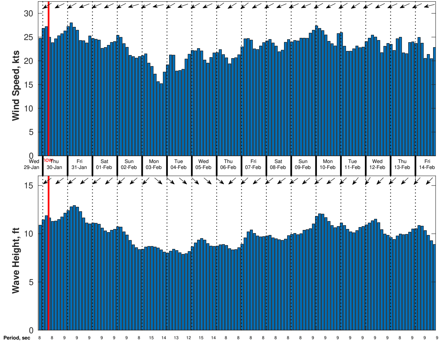
Wind & Wave Forecast for Gyre from 29-Jan-2025 20:00:00 to 14-Feb-2025 20:00:00
