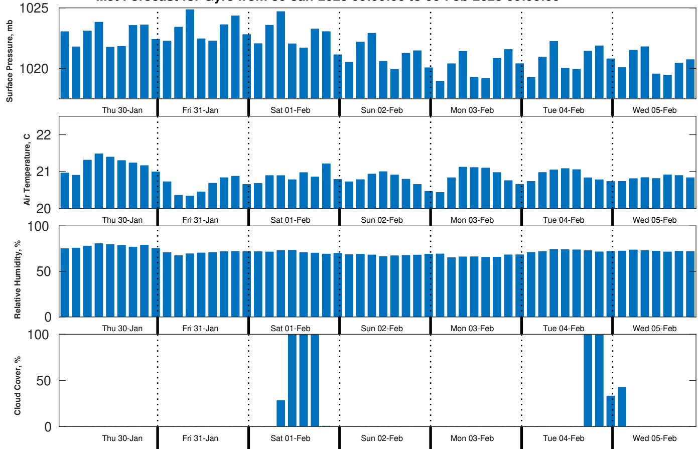
Met Forecast for Gyre from 30-Jan-2025 00:00:00 to 06-Feb-2025 00:00:00
