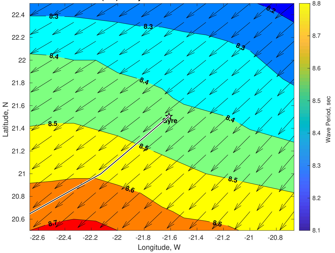
Wave Period (sec) for Gyre at 30-Jan-2025 09:00:00
