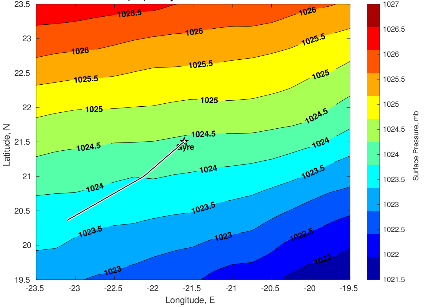
Surface Pressure (mb) for Gyre at 01-Feb-2025 00:00:00
