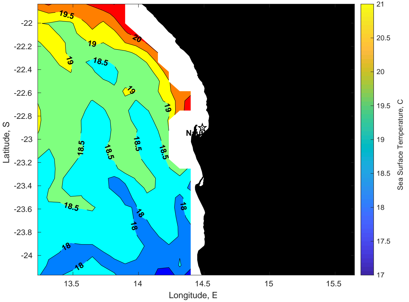
SST for Nautilus at 29-Jan-2025 00:00:00
