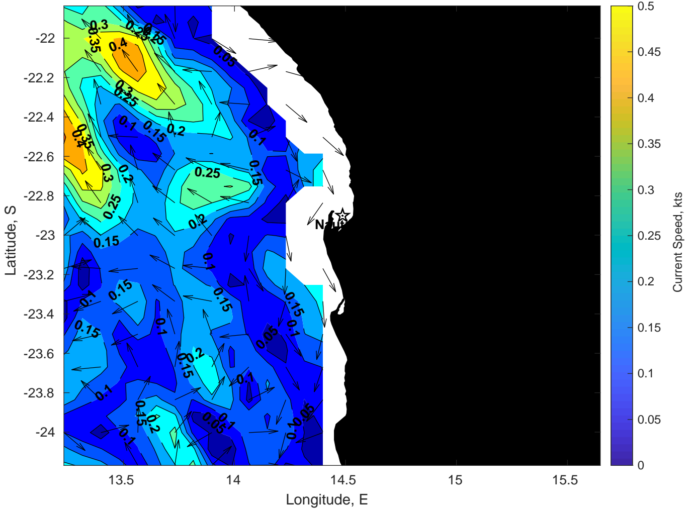
Surface Currents for Nautilus at 29-Jan-2025 00:00:00
