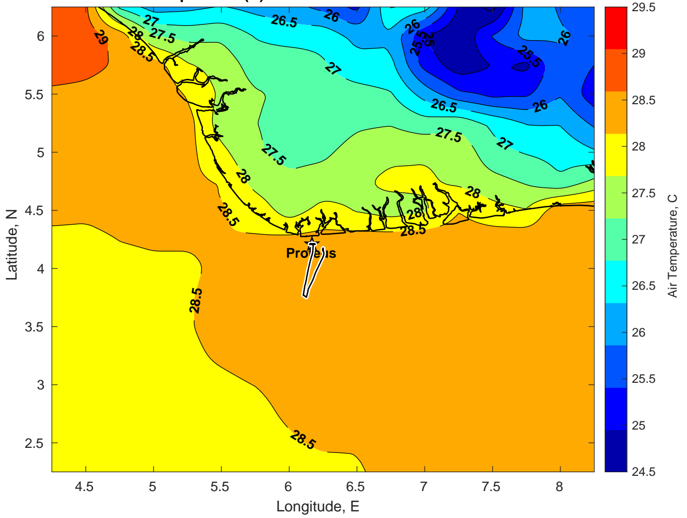
Air Temperature (C) for Proteus at 30-Jan-2025
