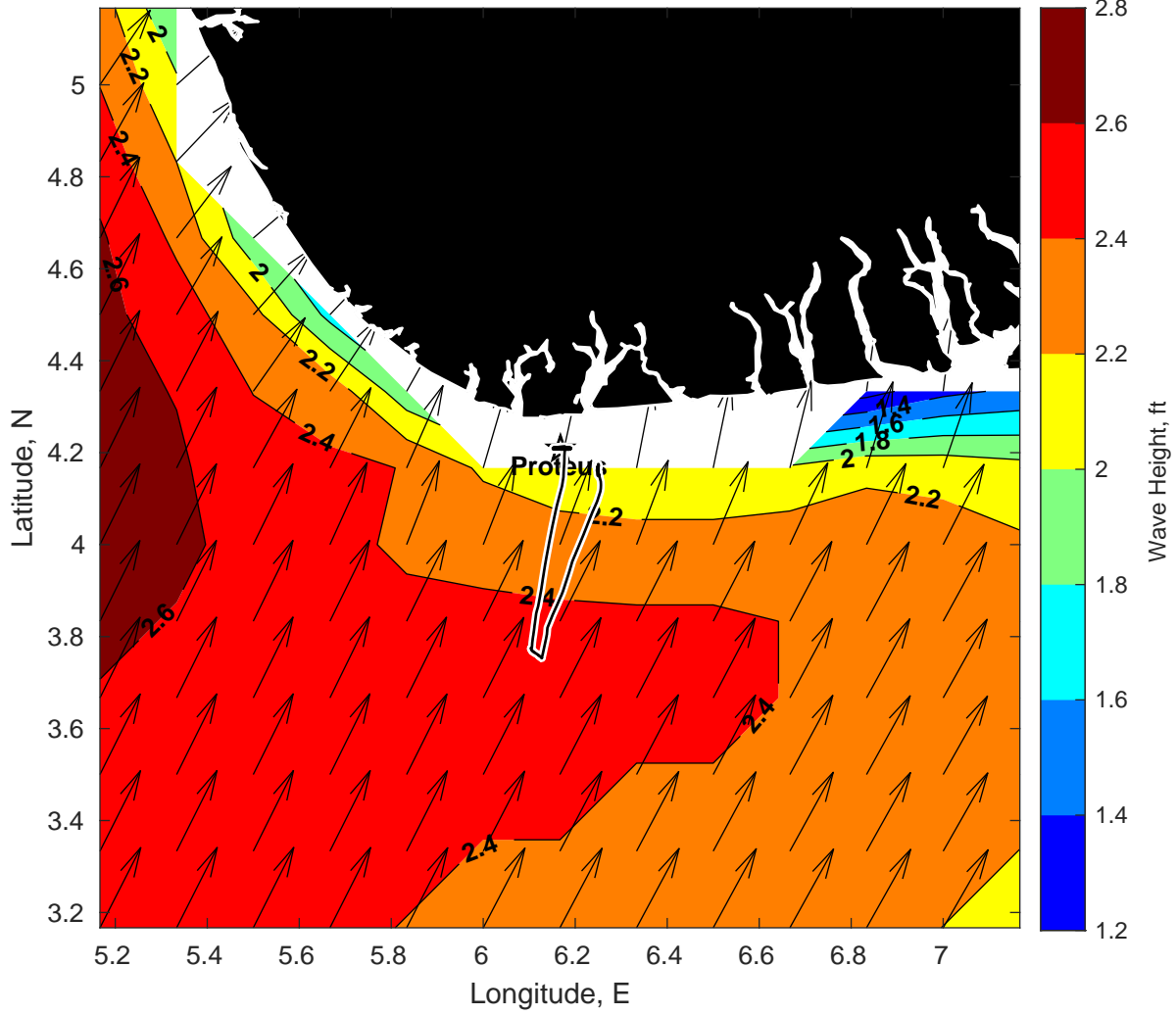
Wave Height (ft) for Proteus at 30-Jan-2025 09:00:00
