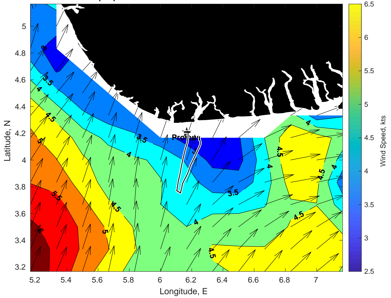
Winds (kts) for Proteus at 30-Jan-2025 09:00:00
