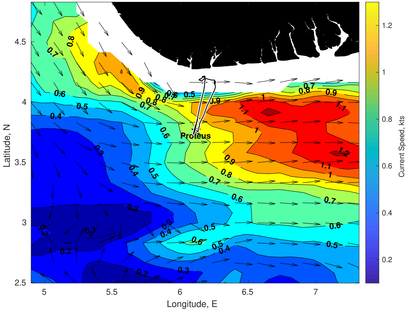
Surface Currents for Proteus at 29-Jan-2025 00:00:00
