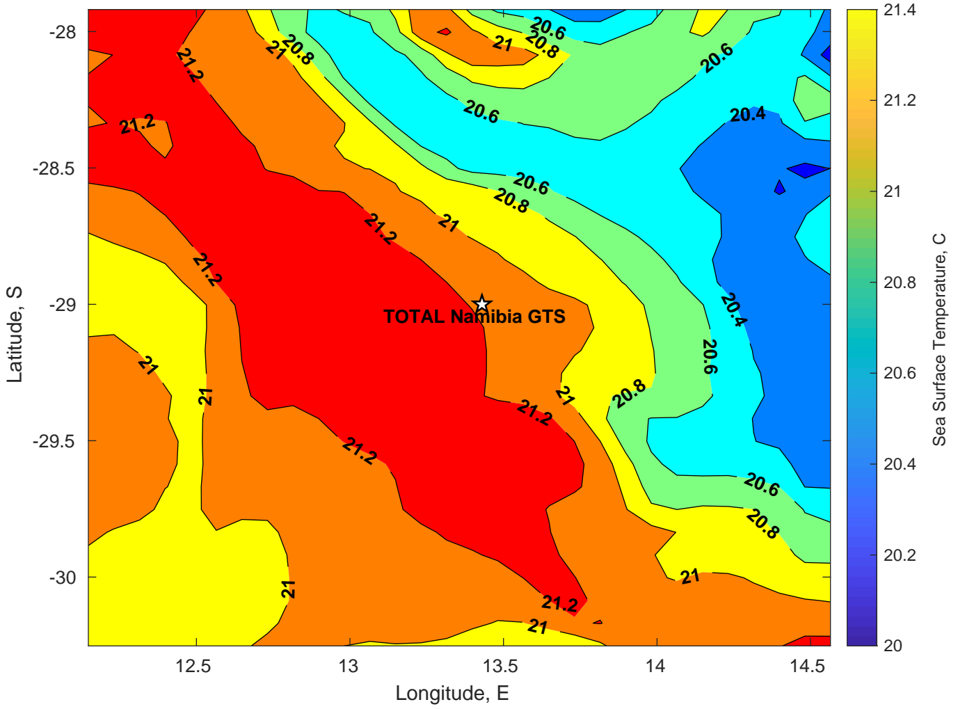
SST for TOTAL Namibia GTS at 29-Jan-2025 00:00:00
