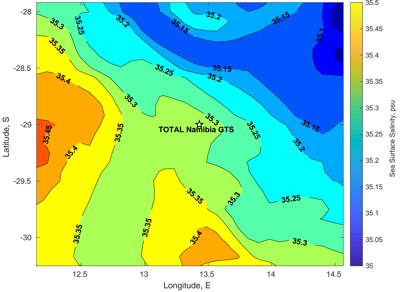
Surface Salinity for TOTAL Namibia GTS at 29-Jan-2025 00:00:00
