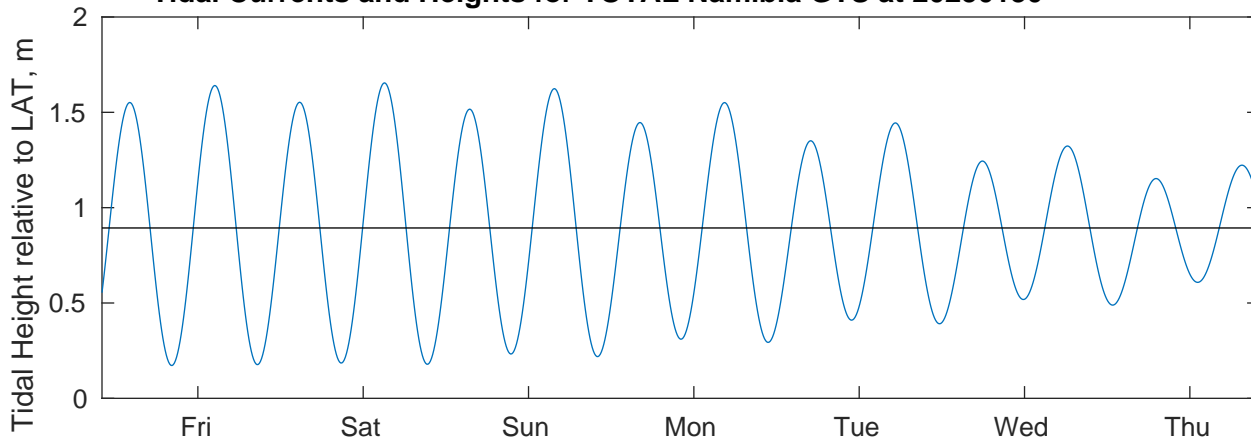
Tidal Currents and Heights for TOTAL Namibia GTS at 20250130
