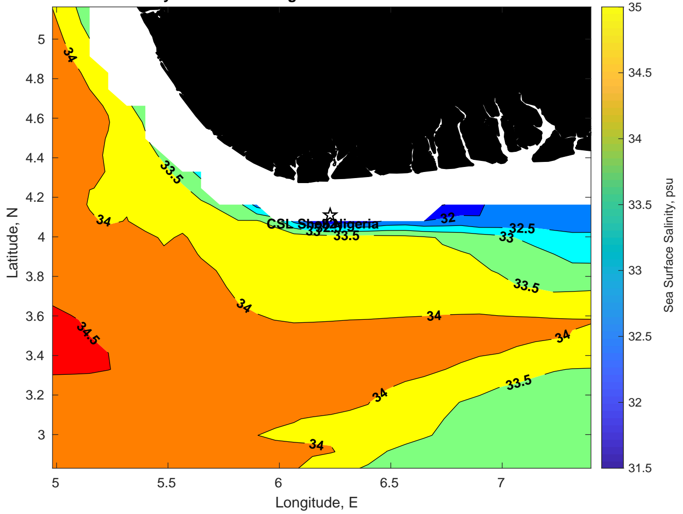
Surface Salinity for CSL Shell Nigeria at 30-Jan-2025 00:00:00
