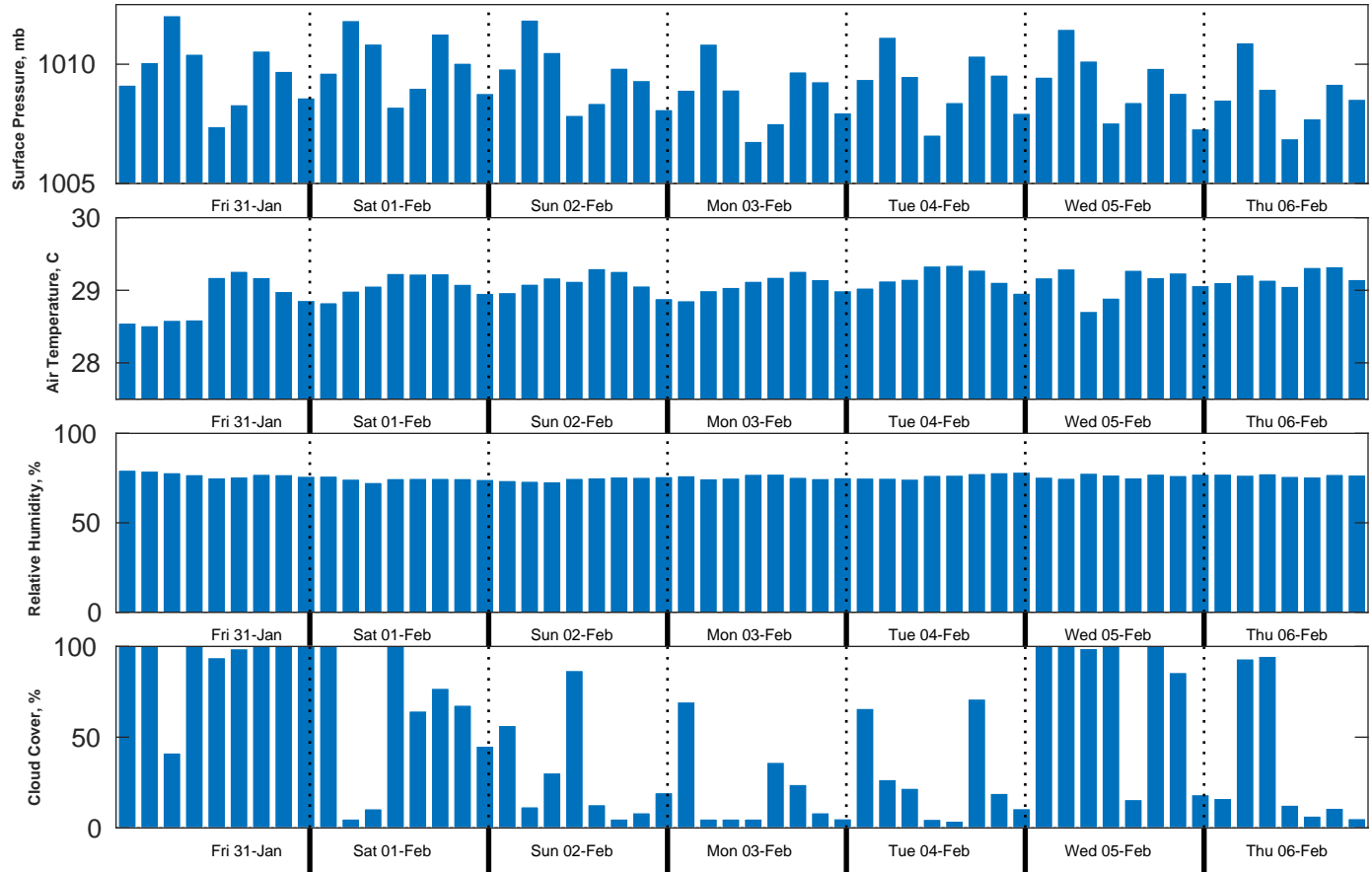
Met Forecast for CSL Shell Nigeria from 31-Jan-2025 00:00:00 to 07-Feb-2025 00:00:00
