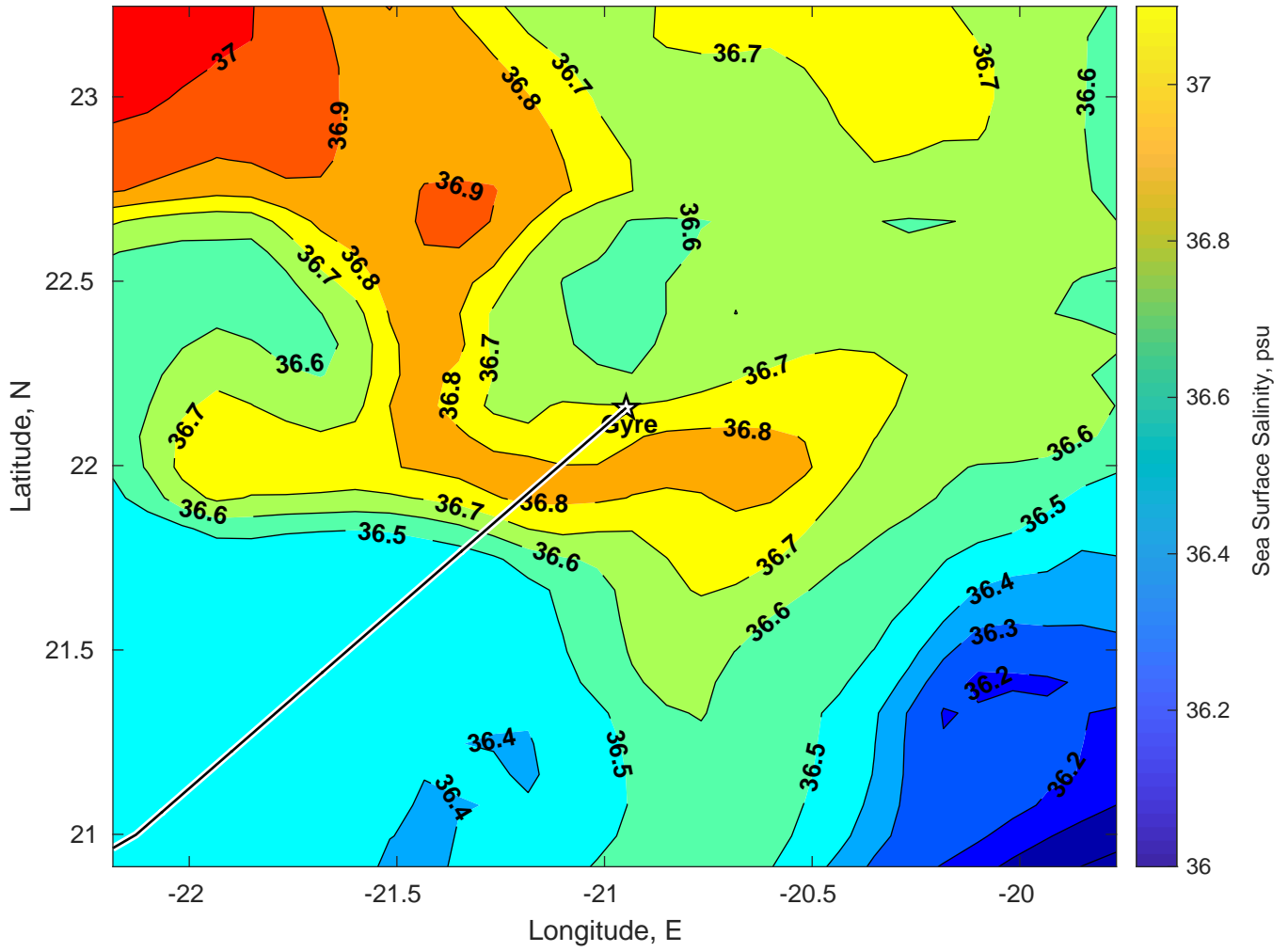
Surface Salinity for Gyre at 30-Jan-2025 00:00:00
