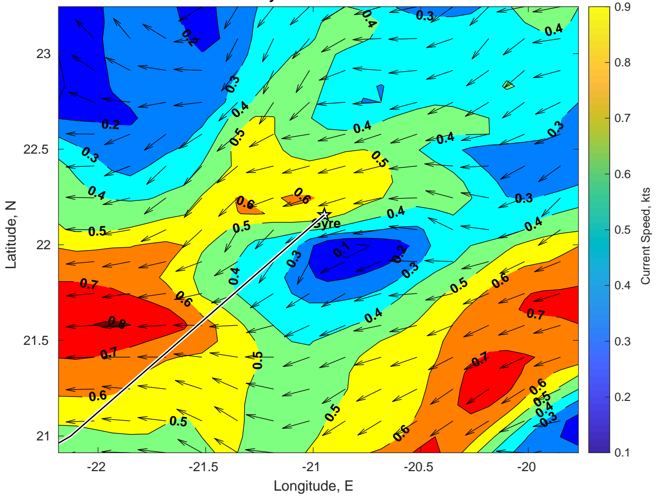
Surface Currents for Gyre at 30-Jan-2025 00:00:00
