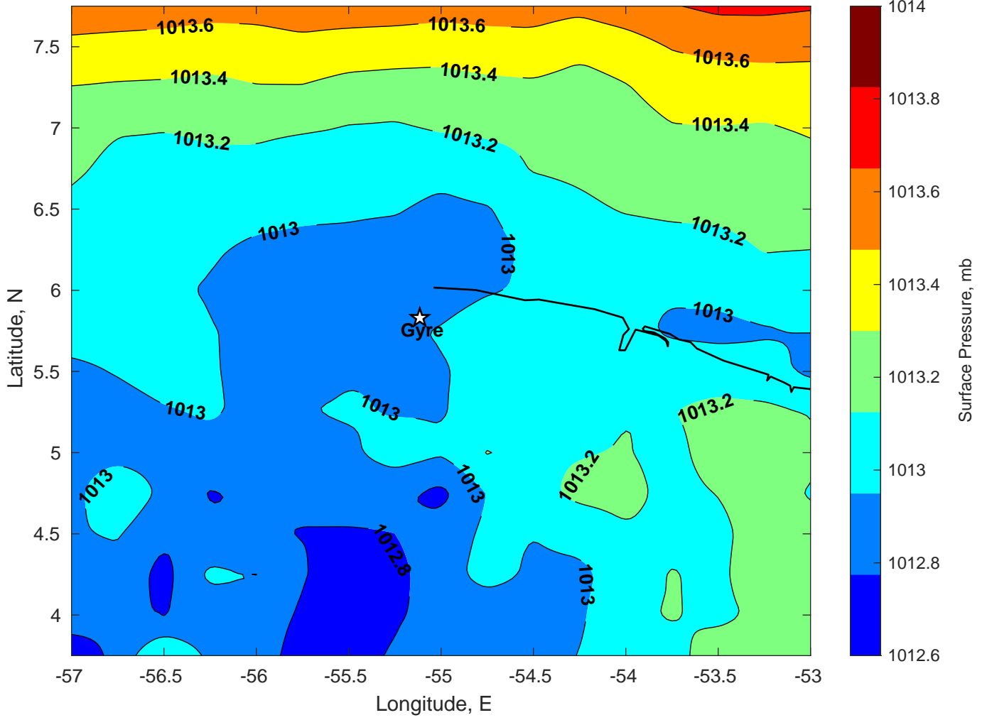
Surface Pressure (mb) for Gyre at 31-Jan-2025 00:00:00
