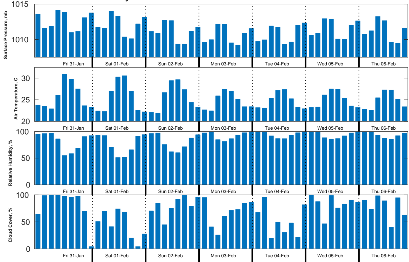
Met Forecast for Gyre from 31-Jan-2025 00:00:00 to 07-Feb-2025 00:00:00
