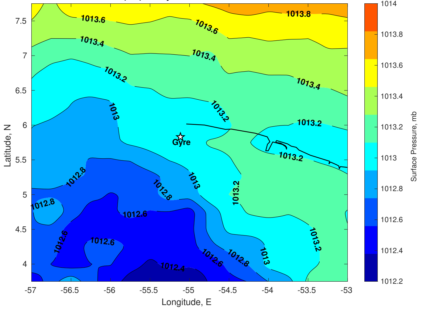
Surface Pressure (mb) for Gyre at 01-Feb-2025 00:00:00
