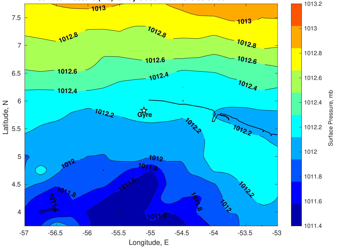
Surface Pressure (mb) for Gyre at 02-Feb-2025 00:00:00
