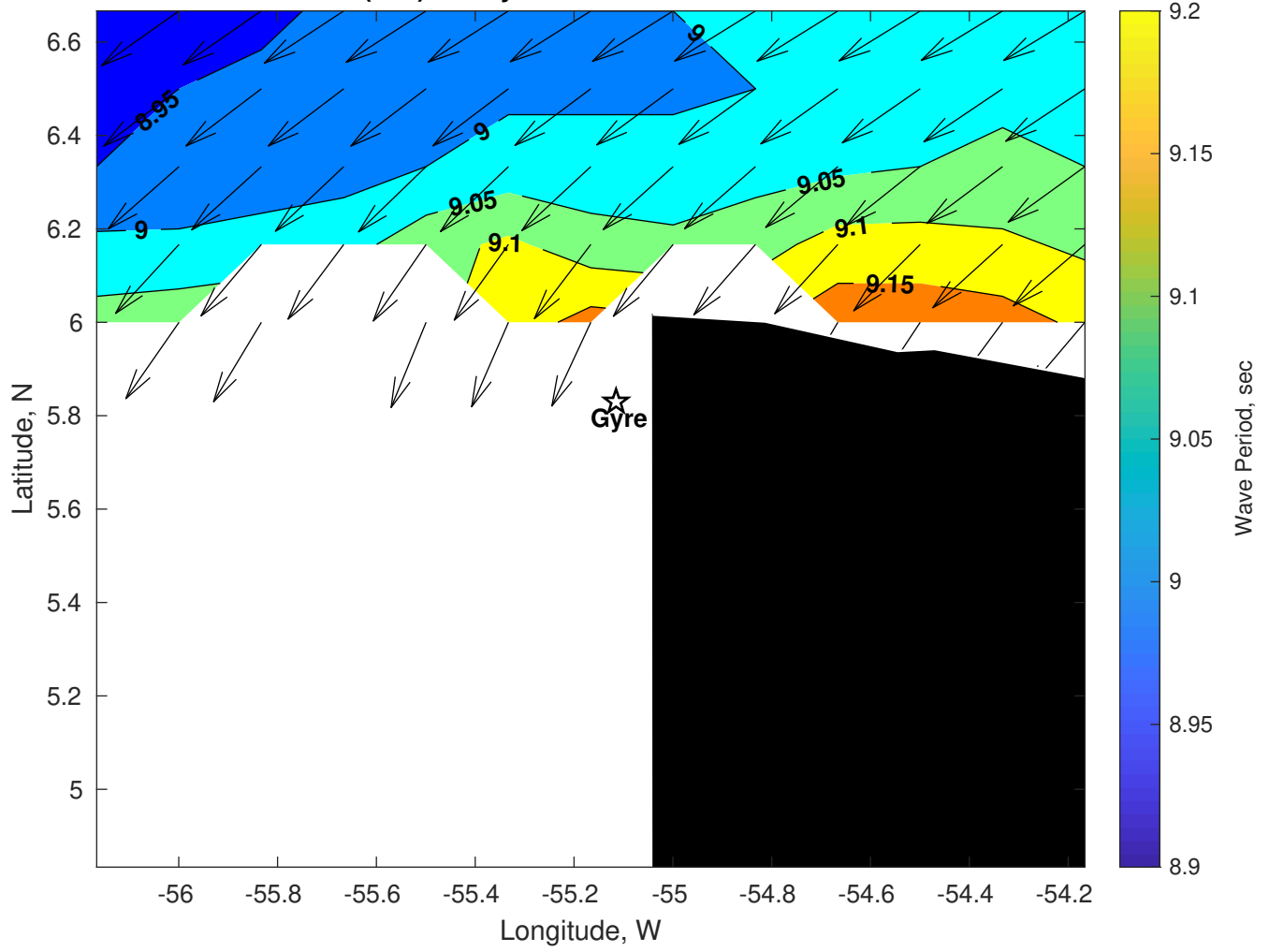
Wave Period (sec) for Gyre at 31-Jan-2025 09:00:00
