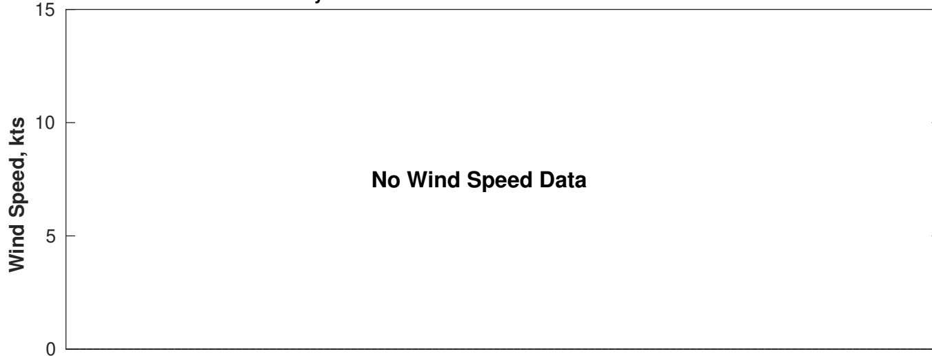
Wind & Wave Forecast for Gyre from 30-Jan-2025 20:00:00 to 15-Feb-2025 20:00:00
