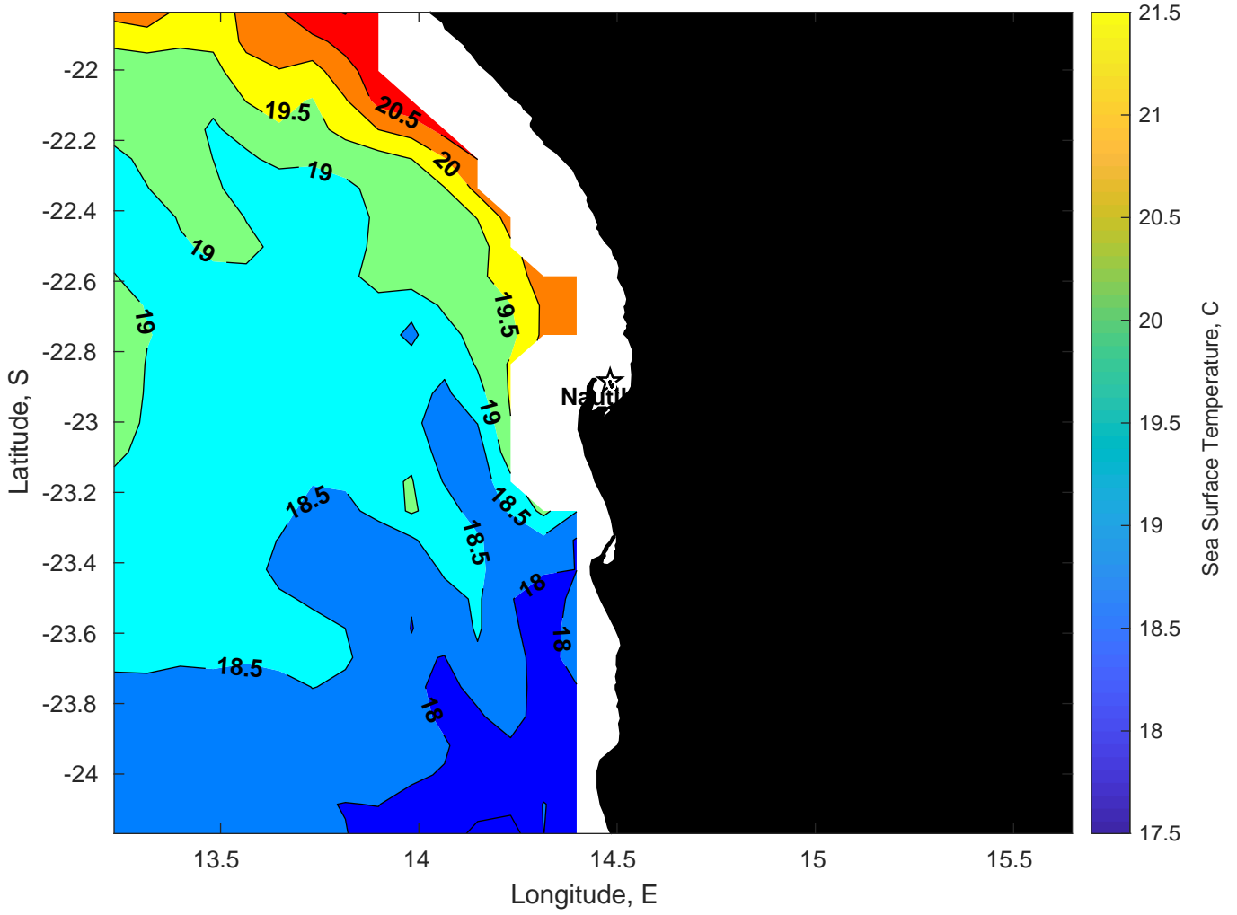
SST for Nautilus at 30-Jan-2025 00:00:00
