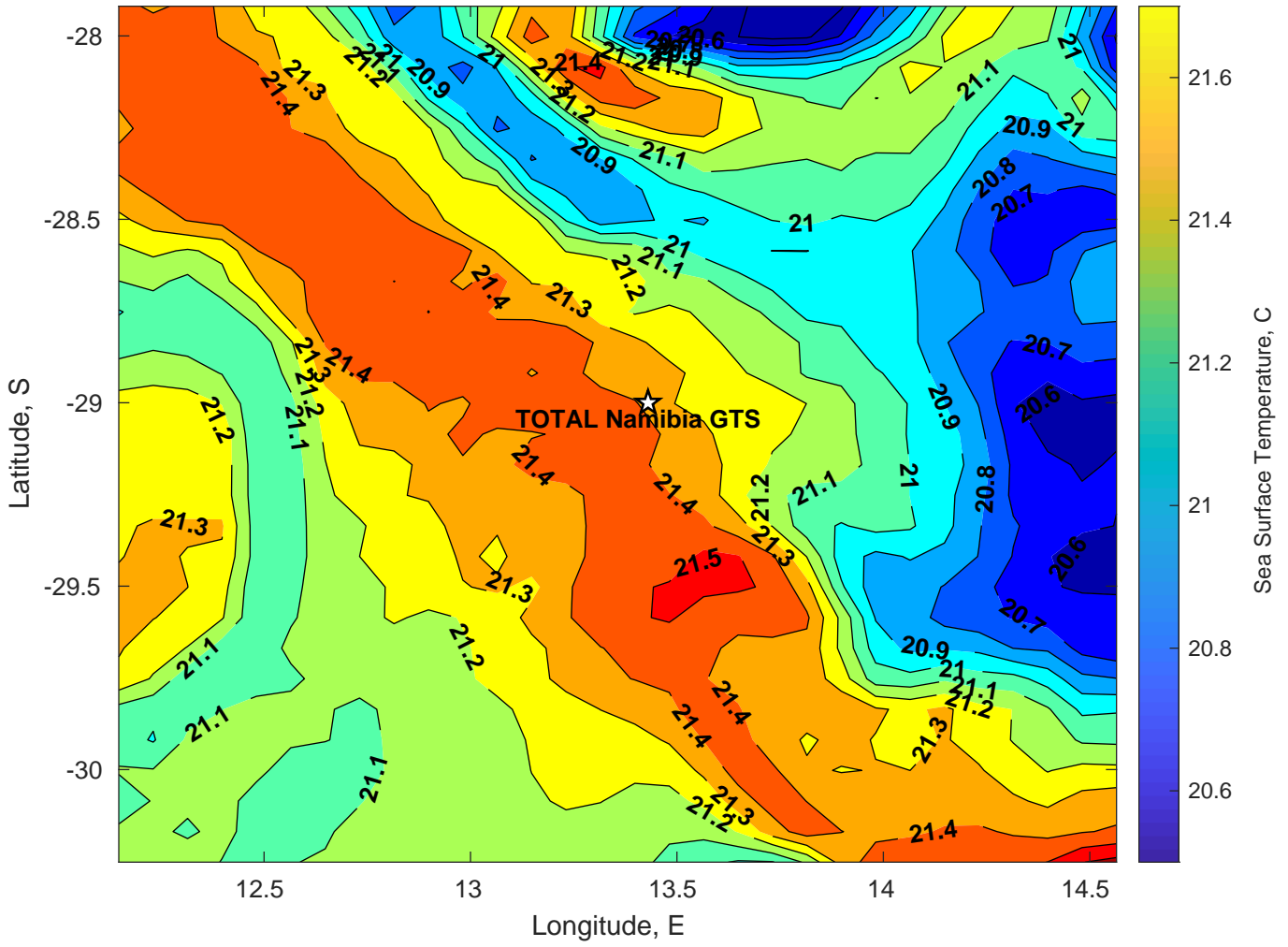
SST for TOTAL Namibia GTS at 30-Jan-2025 00:00:00
