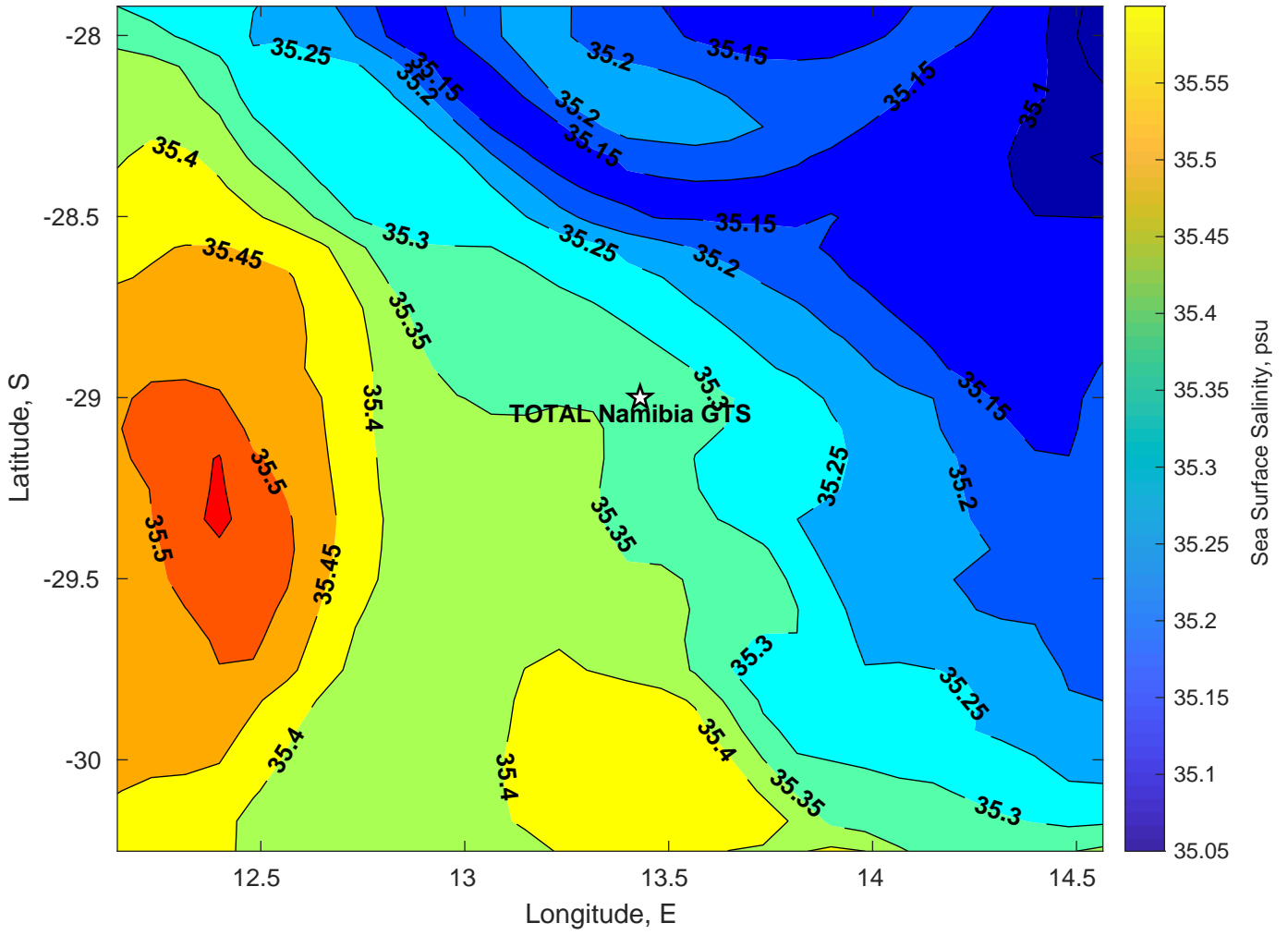
Surface Salinity for TOTAL Namibia GTS at 30-Jan-2025 00:00:00
