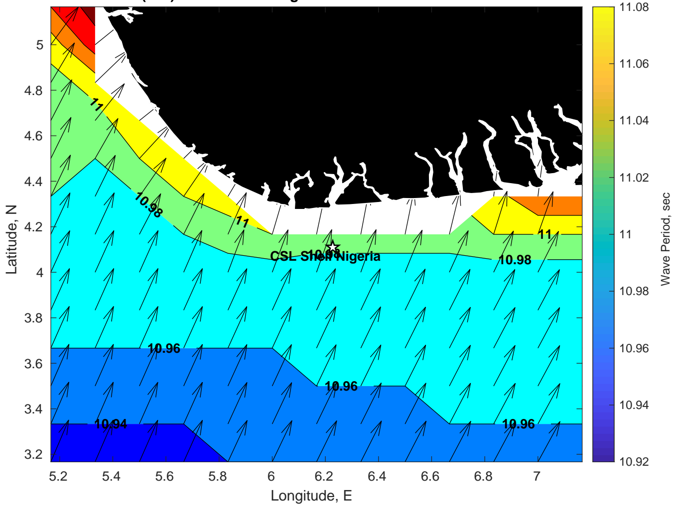
Wave Period (sec) for CSL Shell Nigeria at 31-Jan-2025 21:00:00
