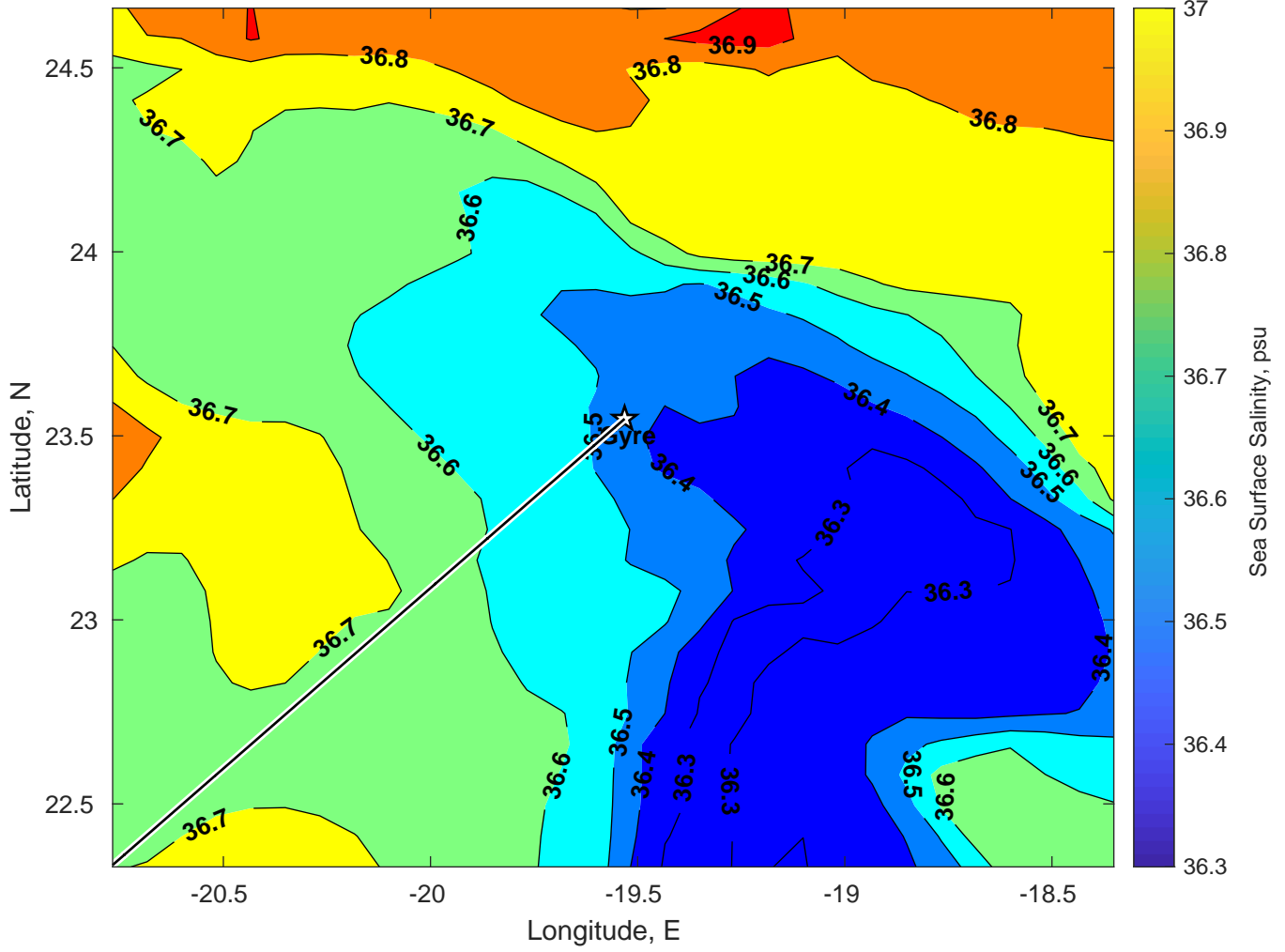
Surface Salinity for Gyre at 31-Jan-2025 00:00:00
