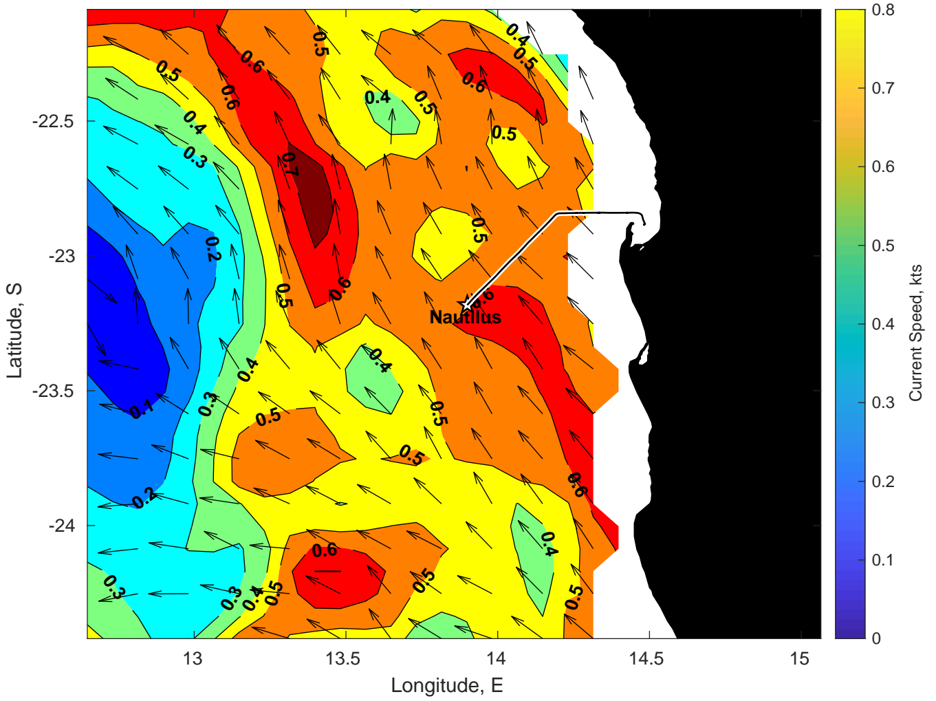
Surface Currents for Nautilus at 31-Jan-2025 00:00:00
