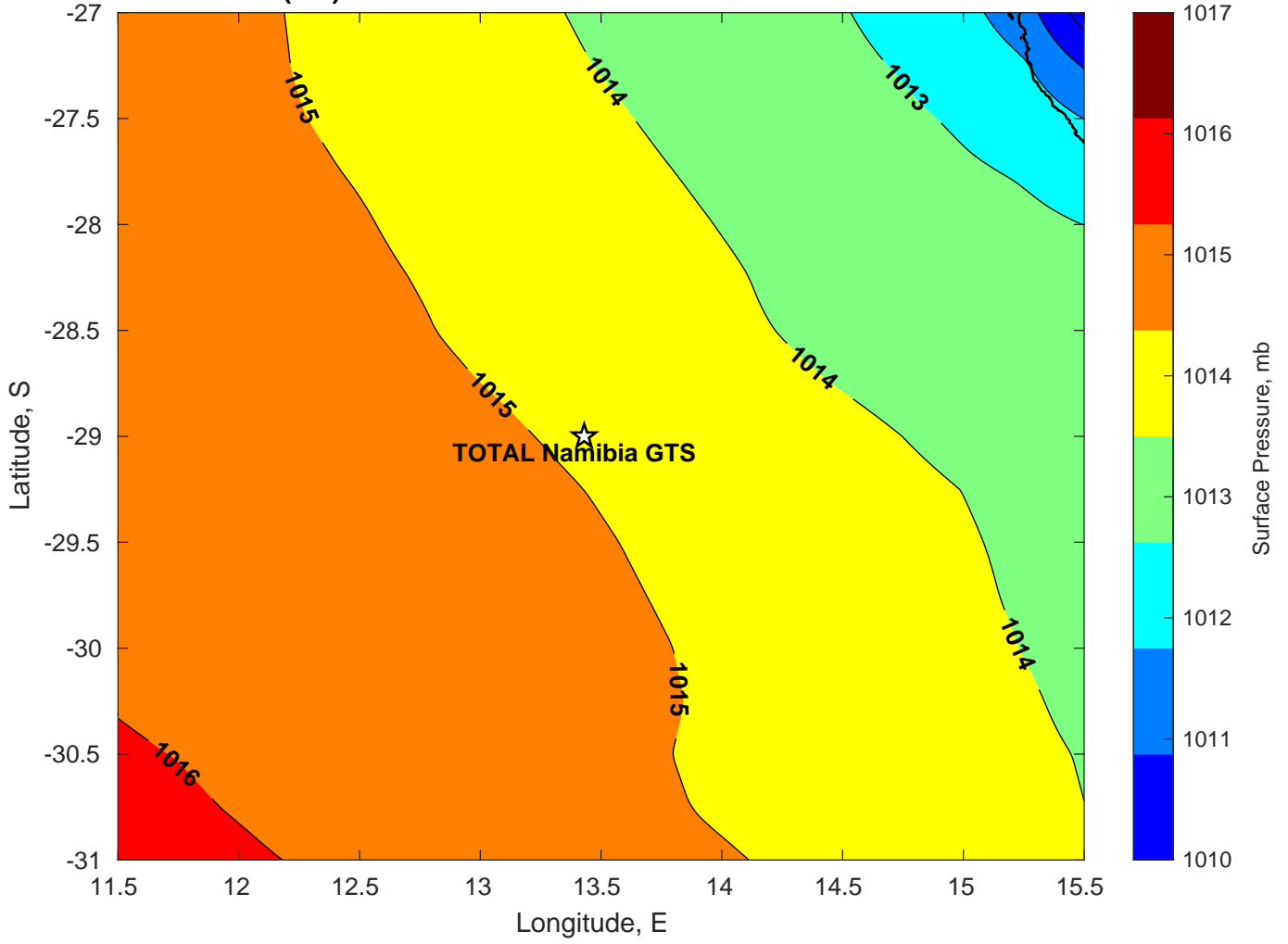
Surface Pressure (mb) for TOTAL Namibia GTS at 01-Feb-2025 12:00:00
