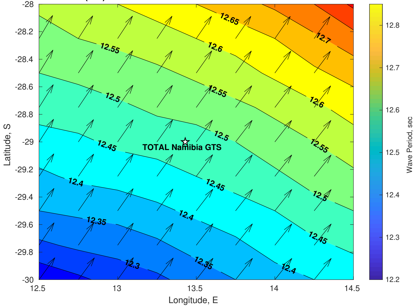
Wave Period (sec) for TOTAL Namibia GTS at 31-Jan-2025 21:00:00
