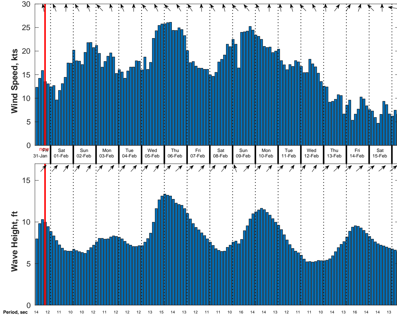
Wind & Wave Forecast for TOTAL Namibia GTS from 31-Jan-2025 08:00:00 to 16-Feb-2025 08:00:00
