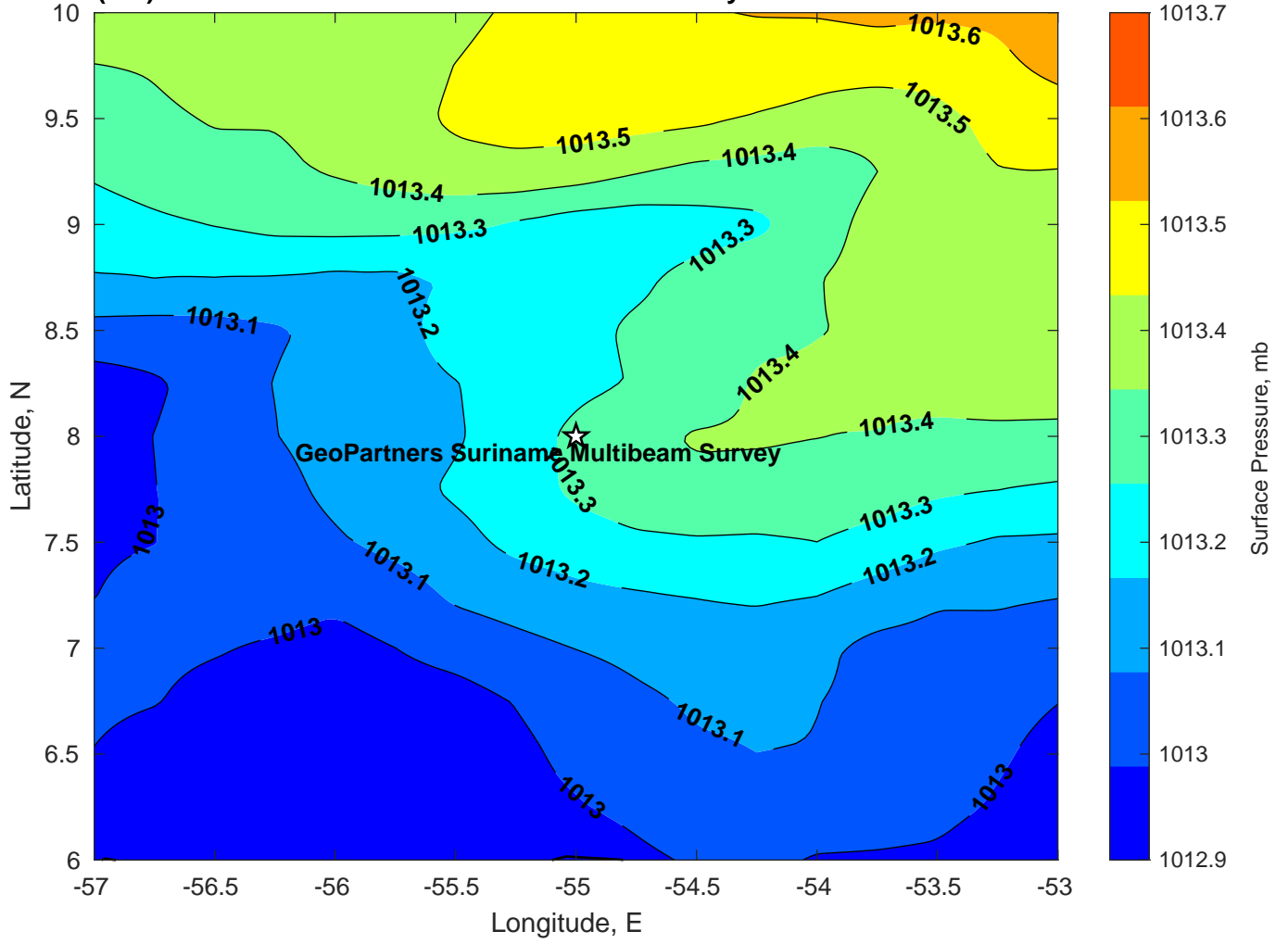
Surface Pressure (mb) for GeoPartners Suriname Multibeam Survey at 10-Jan-2025 12:00:00
