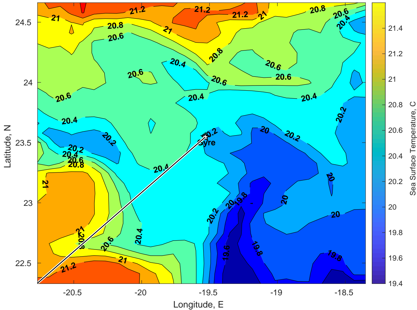
SST for Gyre at 31-Jan-2025 00:00:00
