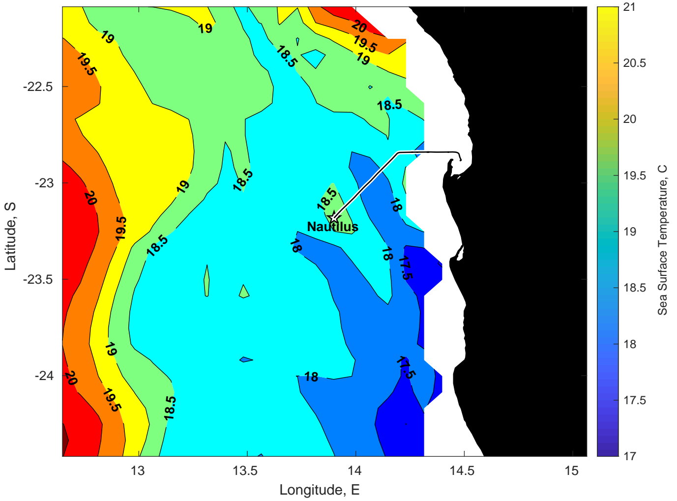
SST for Nautilus at 31-Jan-2025 00:00:00
