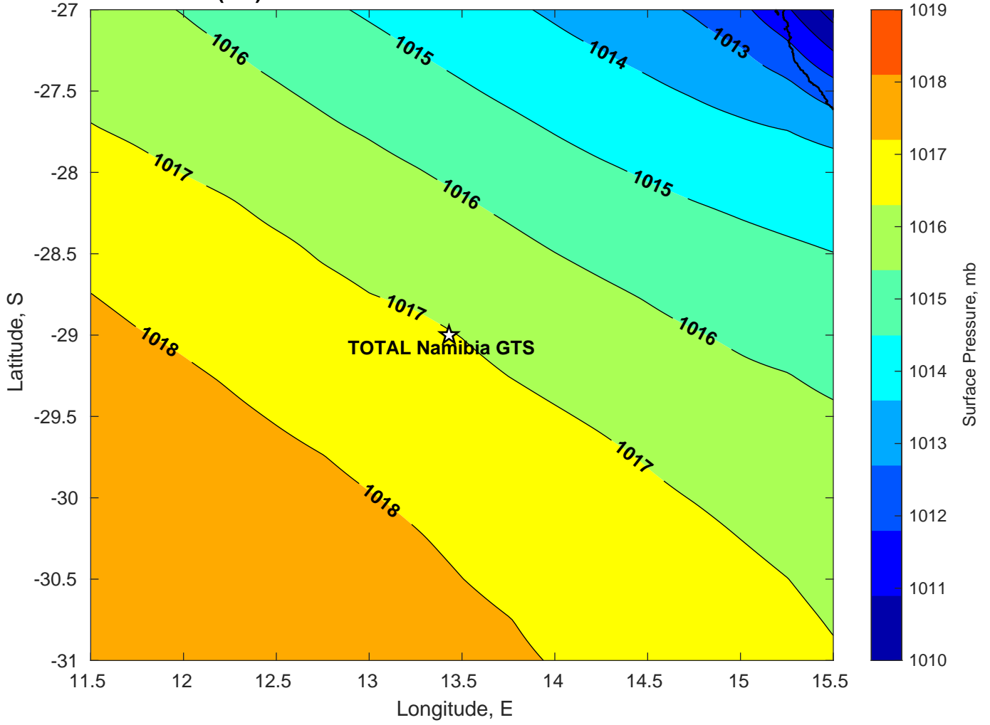
Surface Pressure (mb) for TOTAL Namibia GTS at 02-Feb-2025 12:00:00
