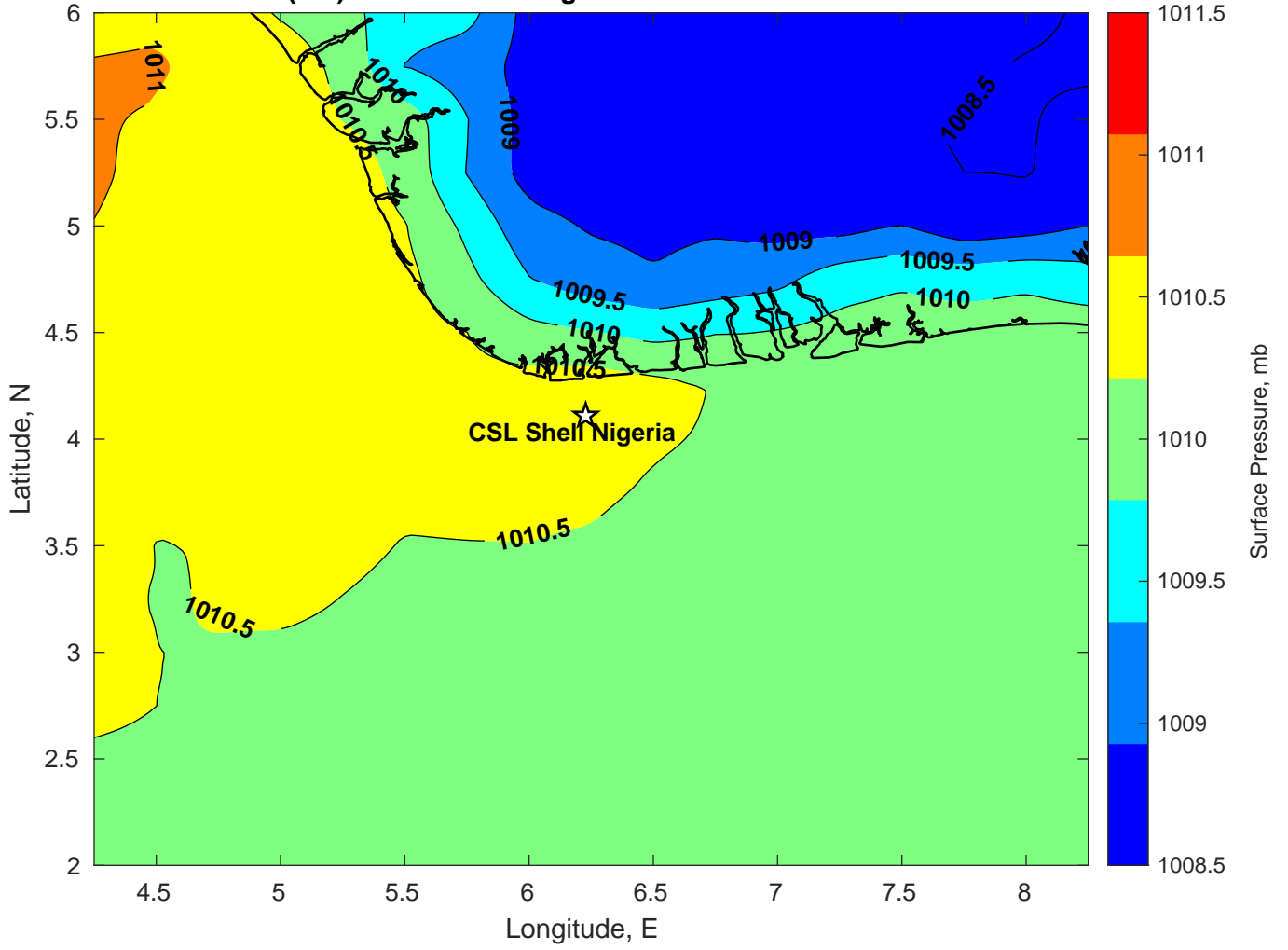
Surface Pressure (mb) for CSL Shell Nigeria at 02-Feb-2025 12:00:00
