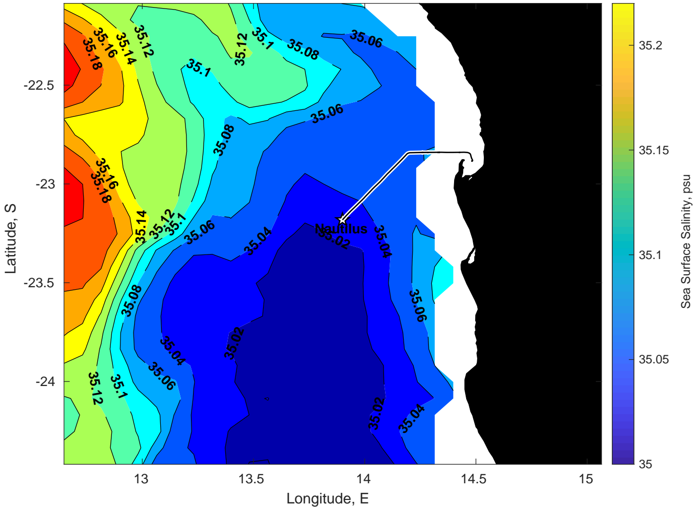
Surface Salinity for Nautilus at 31-Jan-2025 00:00:00
