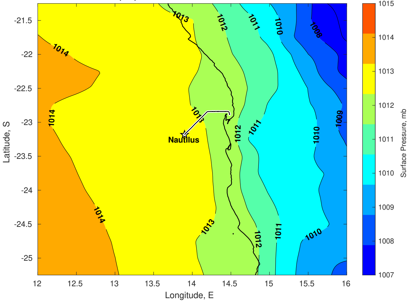
Surface Pressure (mb) for Nautilus at 01-Feb-2025 12:00:00
