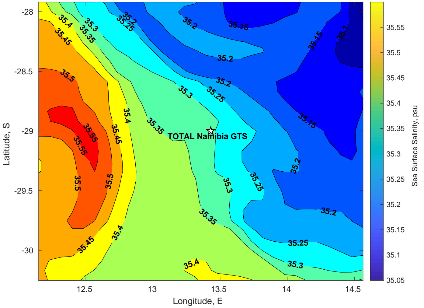
Surface Salinity for TOTAL Namibia GTS at 31-Jan-2025 00:00:00
