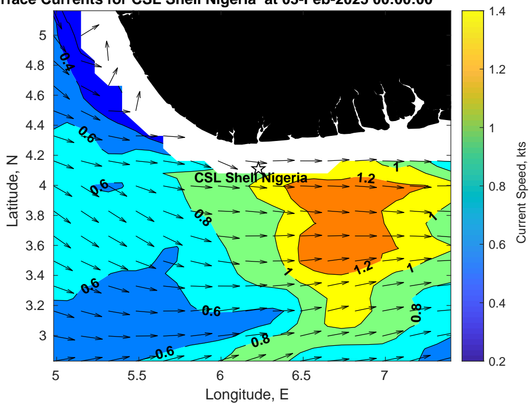
Surface Currents for CSL Shell Nigeria at 03-Feb-2025 00:00:00
