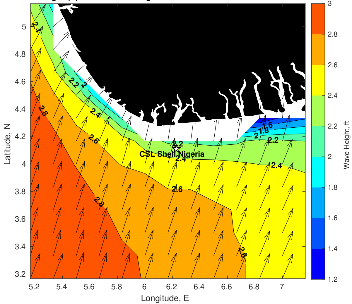
Wave Height (ft) for CSL Shell Nigeria at 04-Feb-2025 09:00:00
