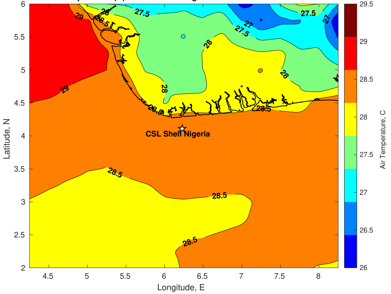
Air Temperature (C) for CSL Shell Nigeria at 04-Feb-2025
