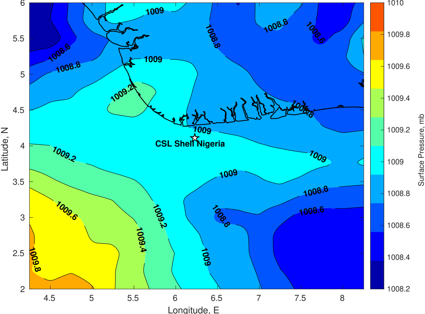
Surface Pressure (mb) for CSL Shell Nigeria at 05-Feb-2025 00:00:00
