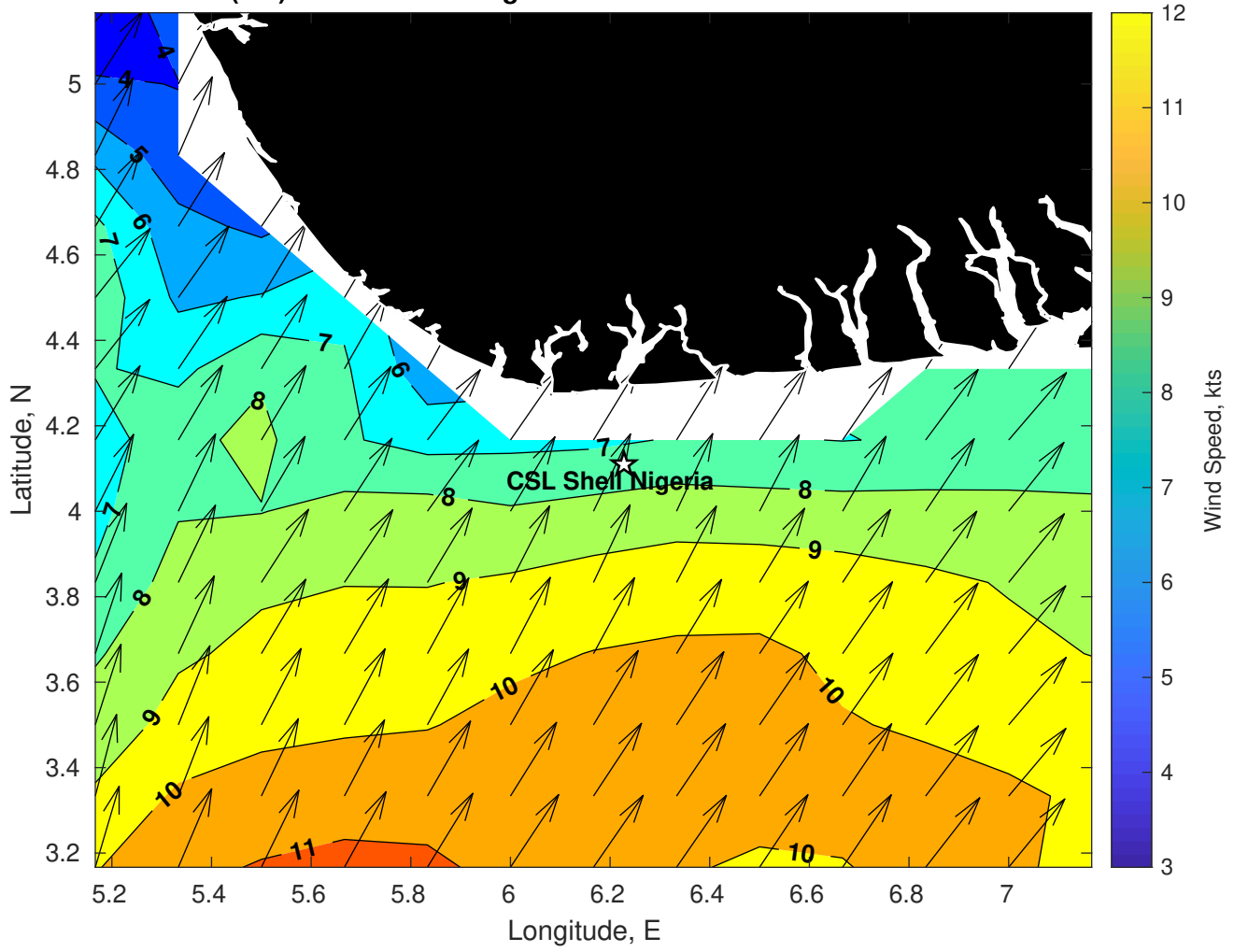
Winds (kts) for CSL Shell Nigeria at 04-Feb-2025 09:00:00
