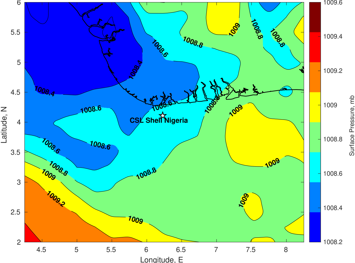
Surface Pressure (mb) for CSL Shell Nigeria at 06-Feb-2025 00:00:00
