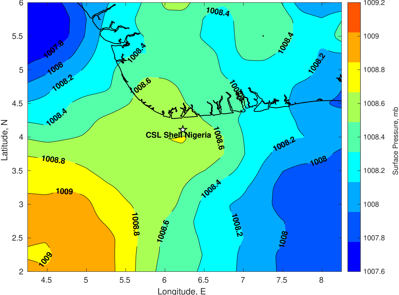
Surface Pressure (mb) for CSL Shell Nigeria at 04-Feb-2025 00:00:00
