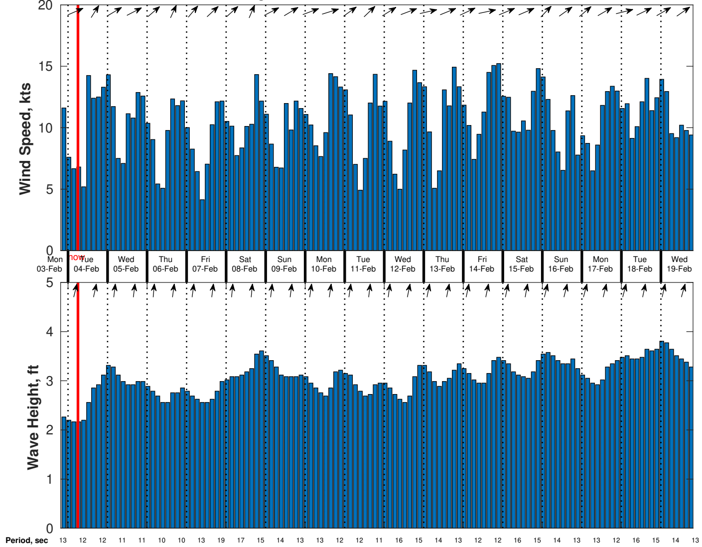
Wind & Wave Forecast for CSL Shell Nigeria from 03-Feb-2025 20:00:00 to 19-Feb-2025 20:00:00
