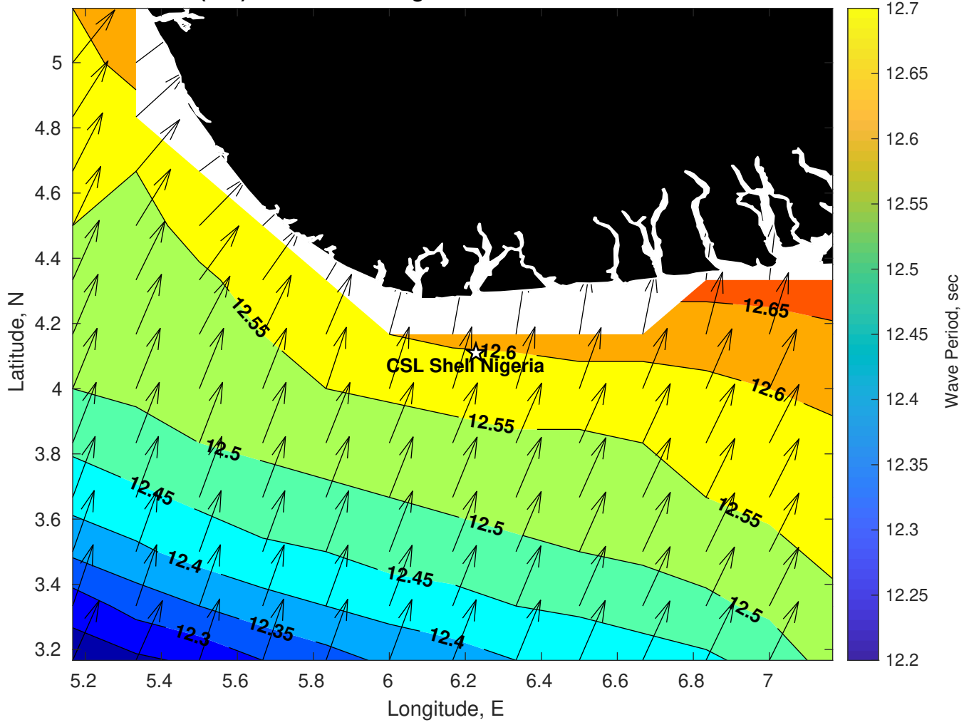
Wave Period (sec) for CSL Shell Nigeria at 04-Feb-2025 09:00:00
