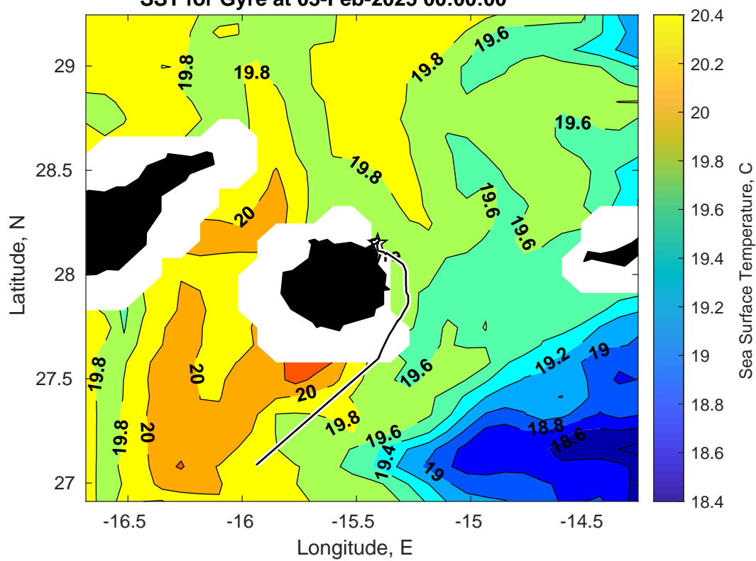
SST for Gyre at 03-Feb-2025 00:00:00
