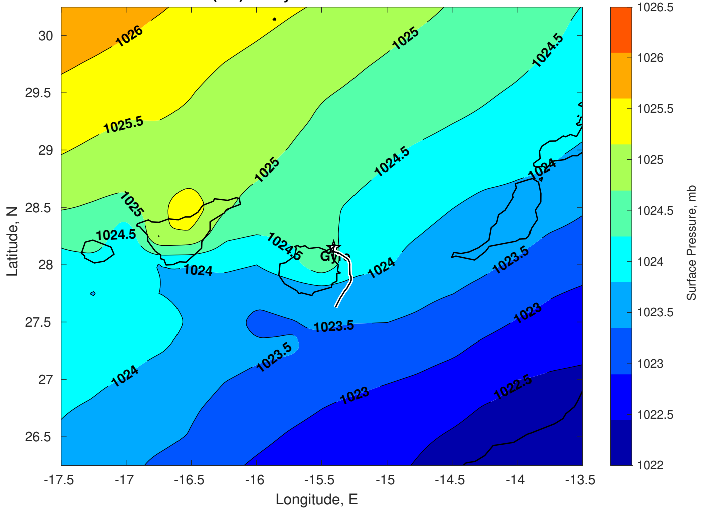
Surface Pressure (mb) for Gyre at 04-Feb-2025 00:00:00
