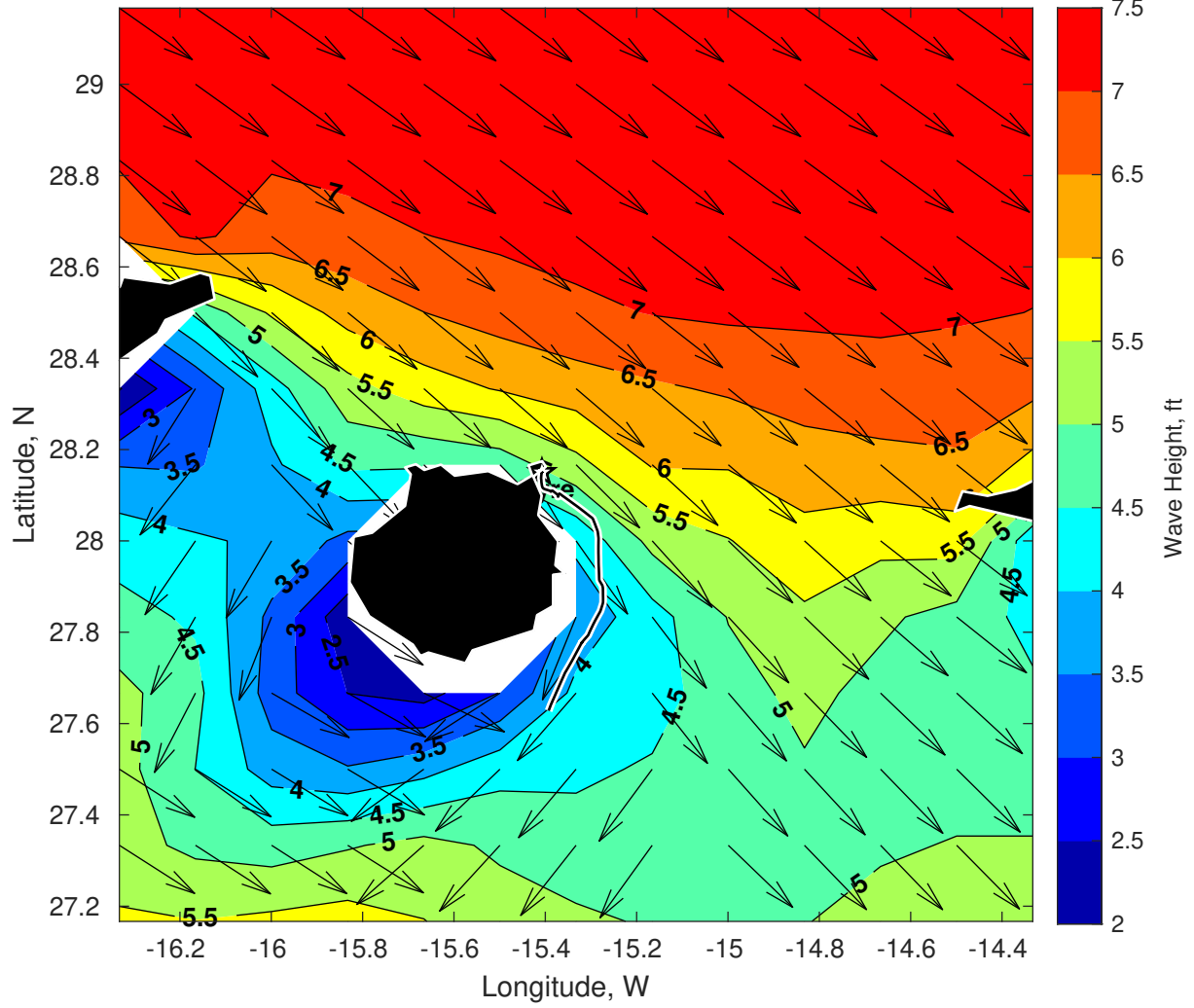
Wave Height (ft) for Gyre at 04-Feb-2025 09:00:00
