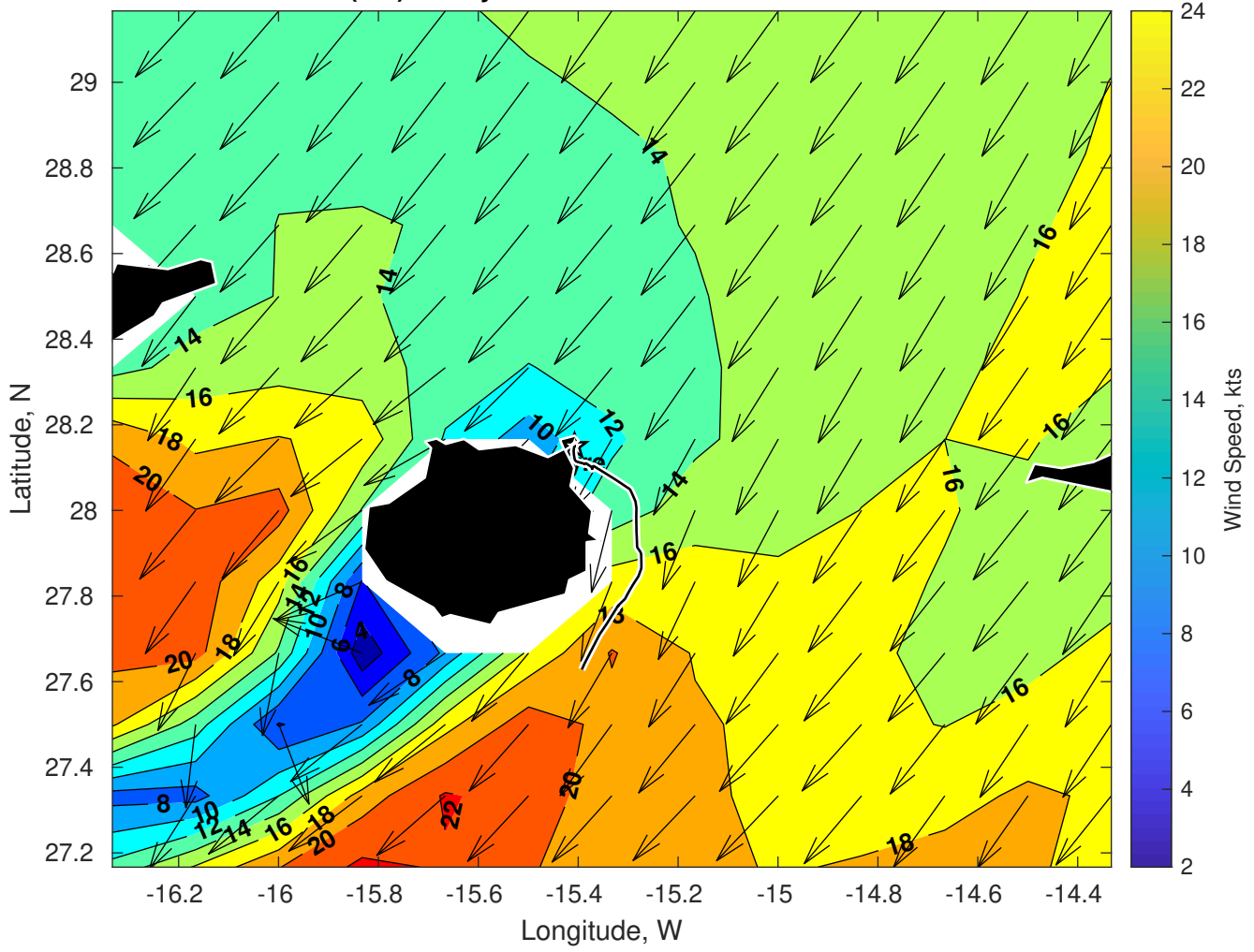
Winds (kts) for Gyre at 04-Feb-2025 09:00:00
