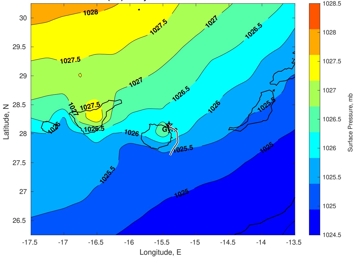
Surface Pressure (mb) for Gyre at 05-Feb-2025 00:00:00
