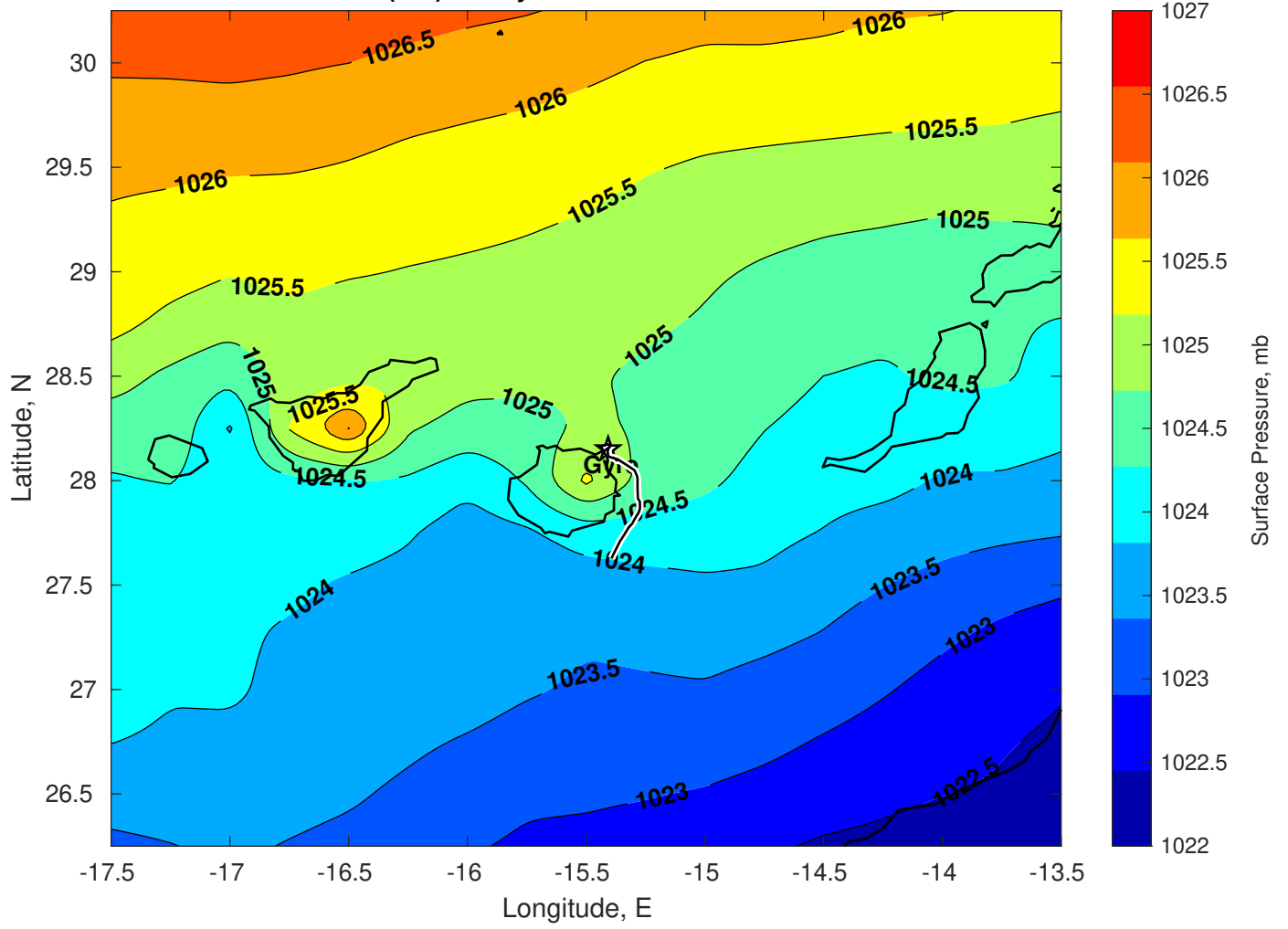
Surface Pressure (mb) for Gyre at 06-Feb-2025 00:00:00
