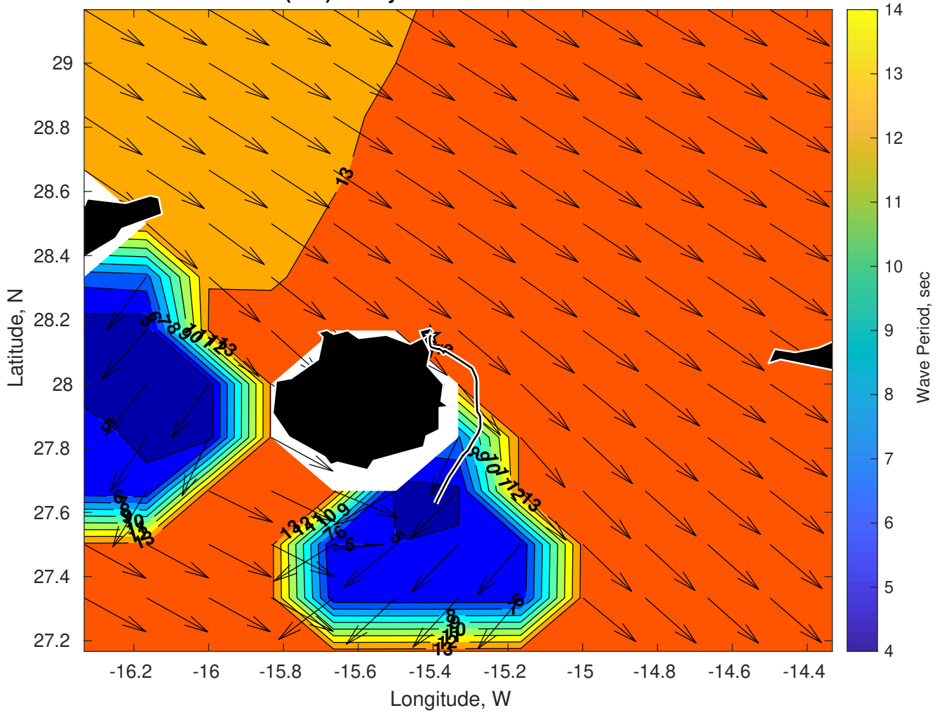
Wave Period (sec) for Gyre at 04-Feb-2025 09:00:00
