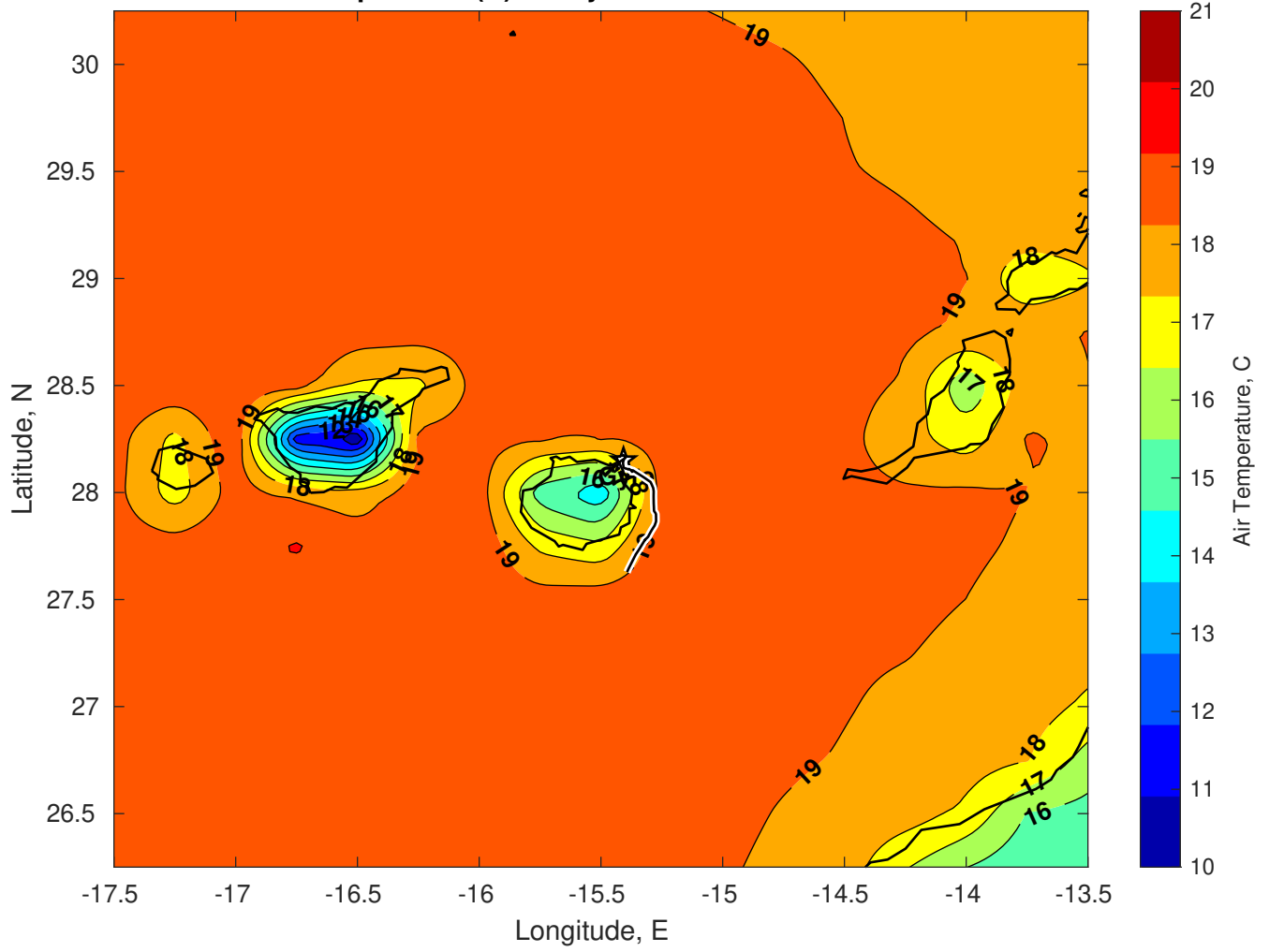
Air Temperature (C) for Gyre at 04-Feb-2025
