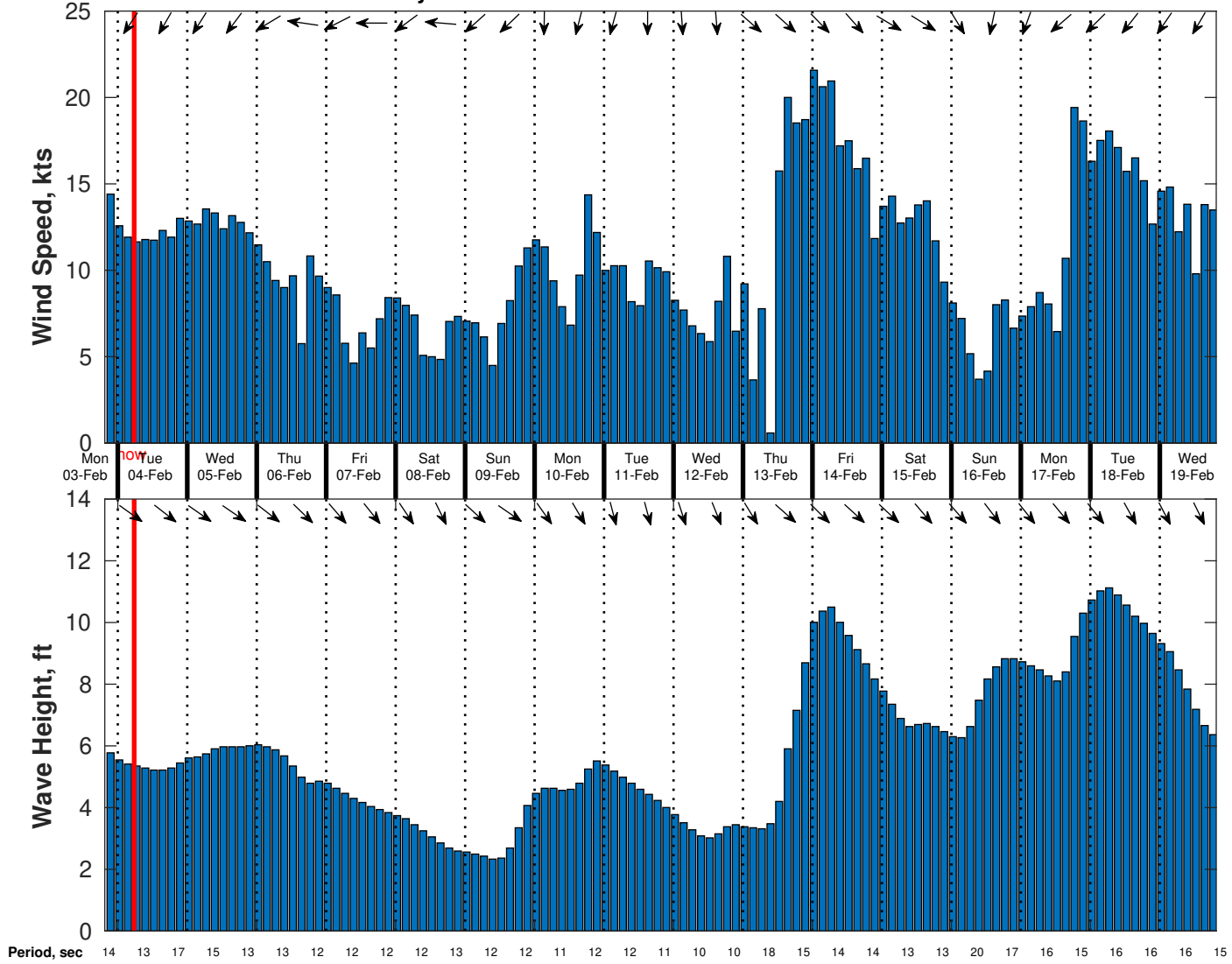
Wind & Wave Forecast for Gyre from 03-Feb-2025 20:00:00 to 19-Feb-2025 20:00:00
