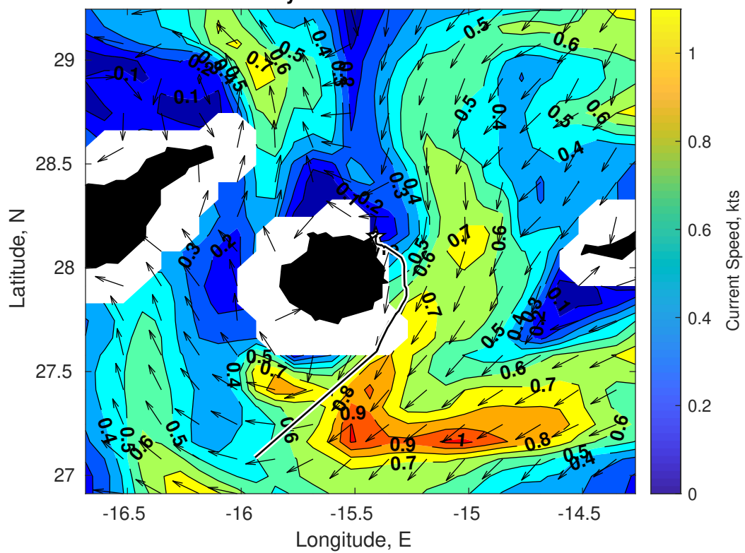
Surface Currents for Gyre at 03-Feb-2025 00:00:00
