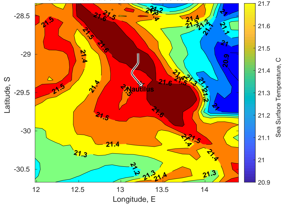
SST for Nautilus at 03-Feb-2025 00:00:00
