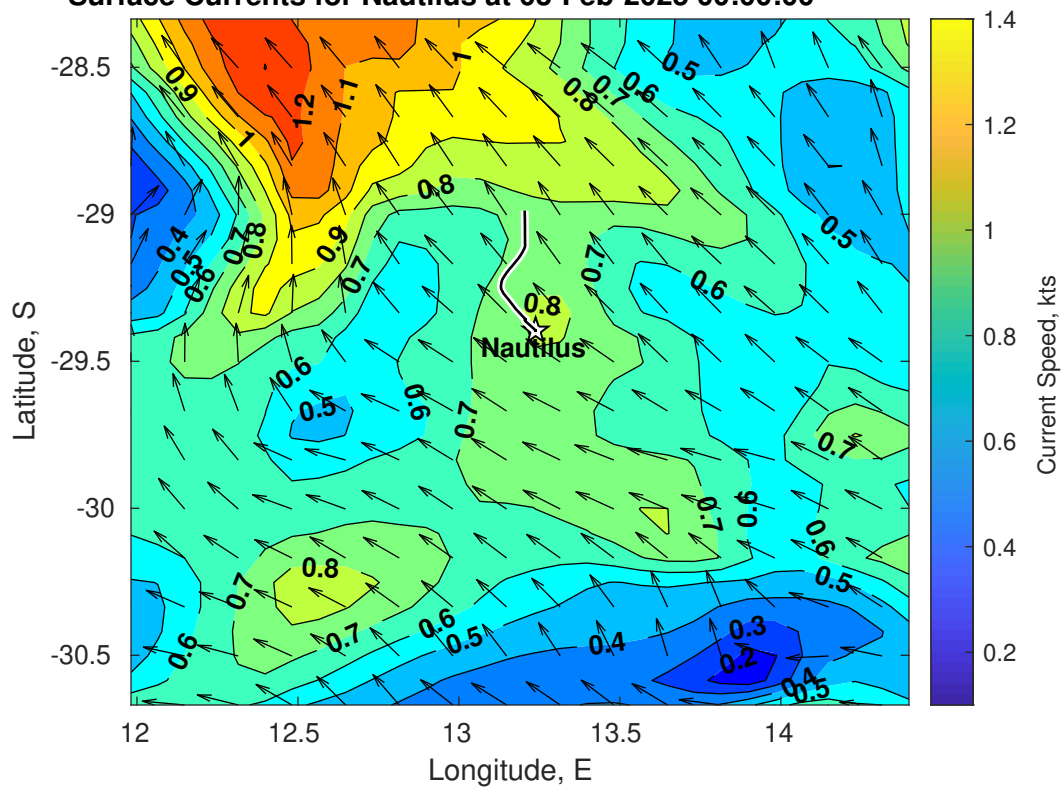
Surface Currents for Nautilus at 03-Feb-2025 00:00:00
