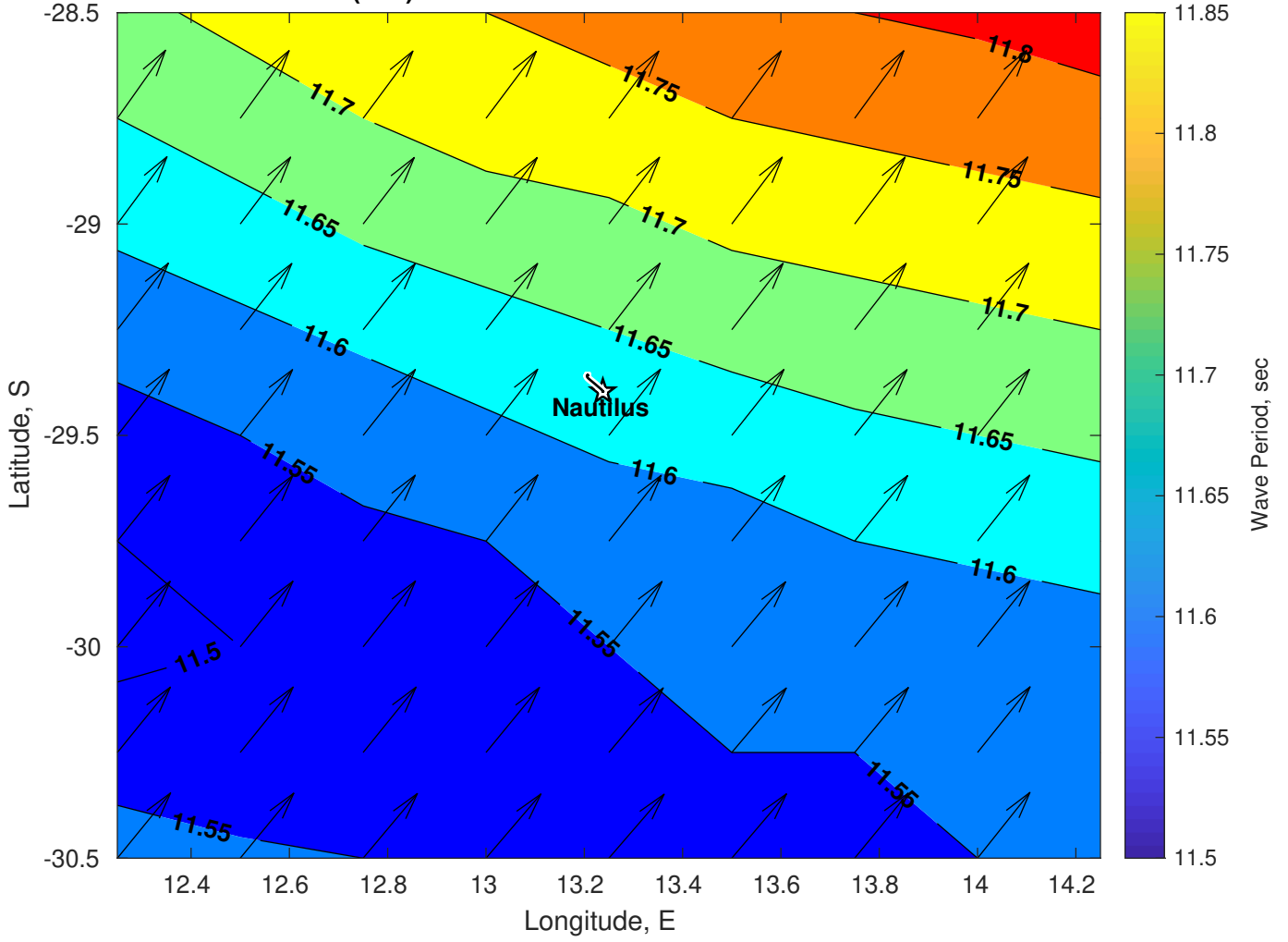
Wave Period (sec) for Nautilus at 04-Feb-2025 09:00:00
