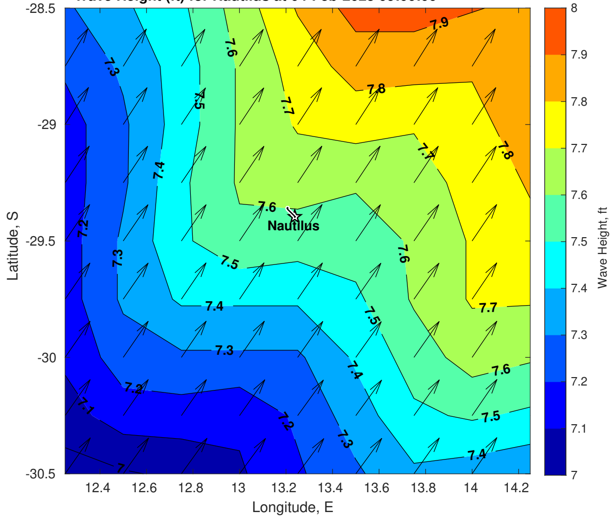
Wave Height (ft) for Nautilus at 04-Feb-2025 09:00:00
