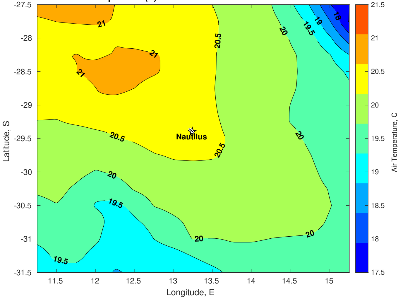
Air Temperature (C) for Nautilus at 04-Feb-2025
