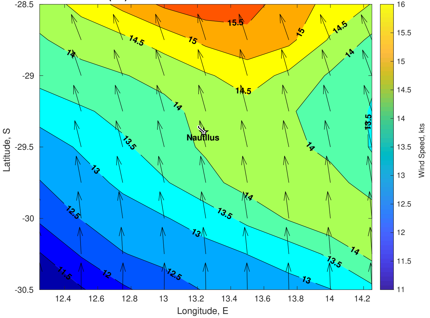
Winds (kts) for Nautilus at 04-Feb-2025 09:00:00
