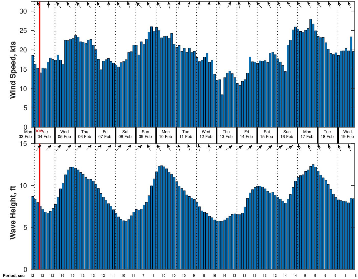
Wind & Wave Forecast for Nautilus from 03-Feb-2025 20:00:00 to 19-Feb-2025 20:00:00
