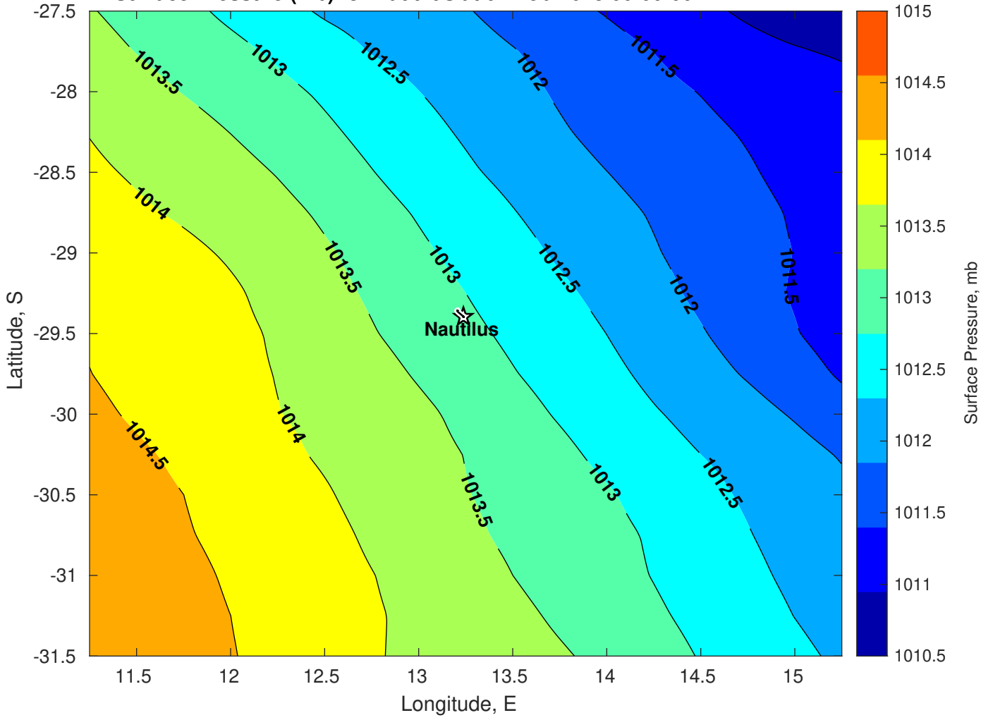
Surface Pressure (mb) for Nautilus at 04-Feb-2025 00:00:00
