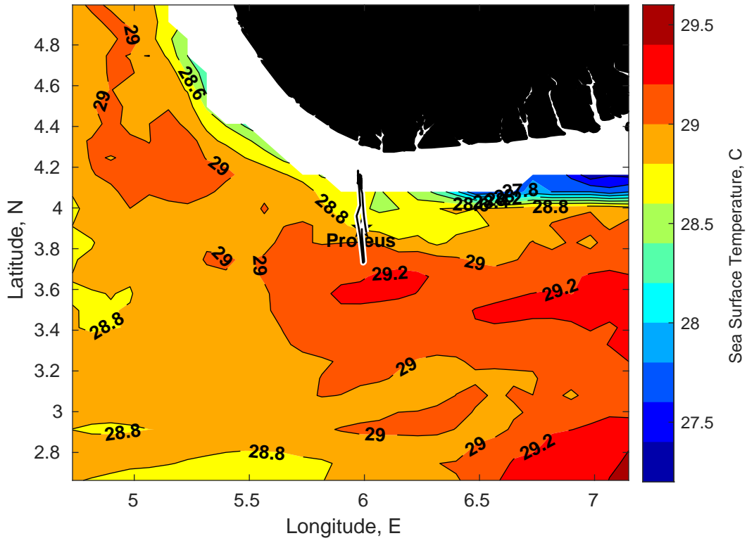
SST for Proteus at 03-Feb-2025 00:00:00
